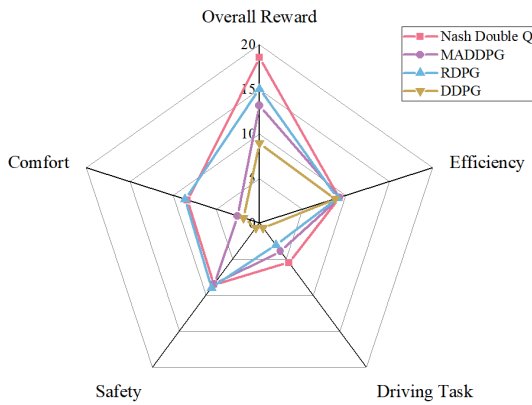
Figure 27: The reward comparisons in second scenario.
