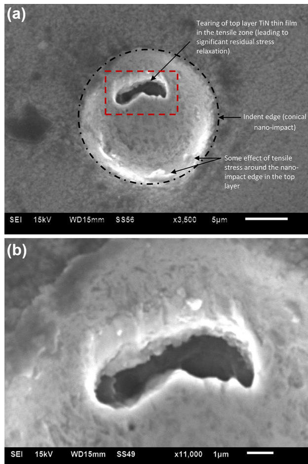
Fig. 9 SEM image of nano-indentation residual impression of functionally graded TiN/TiNi at 100 mN load: a showing some distinct features top layer tearing leading to significant residual stress relaxation, including some other features at the nano-impact edge due to high concentration of impact tensile stresses, and b magnified view of the region ( boxed )
