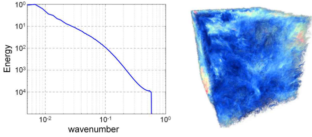
Figure 1: The Kolmogorov spectrum (left) of a 512^3 DNS data set (right) of isotropic turbulence. The color in the direct volume rendering of the isotropic turbulent DNS data set indicates the magnitude of the velocity field with red colors indicating high velocities and blue colors representing low velocities.
