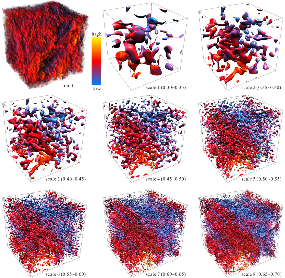
Figure 5: Continuous-scale visualization of turbulence structures in an isotropic turbulent flow. The color indicates the magnitude of the flow velocity, with red and yellow colors indicating large velocities and blue color indicating small velocities.
