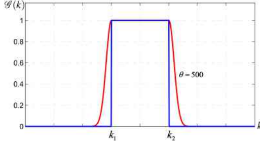
Figure 2: Blue line: perfect band-pass filter (BPF). Red lines: our parameterized filter with two extended fall-off regions.
