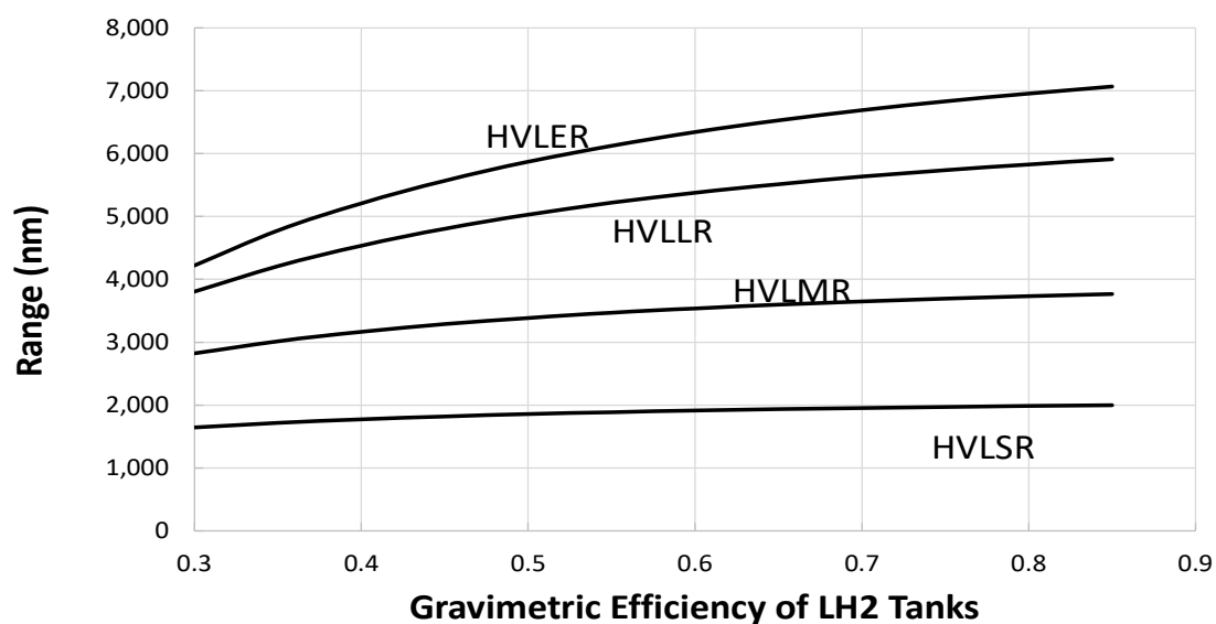
Figure 6 - Impact of liquid hydrogen tank gravimetric efficiency on aircraft range
