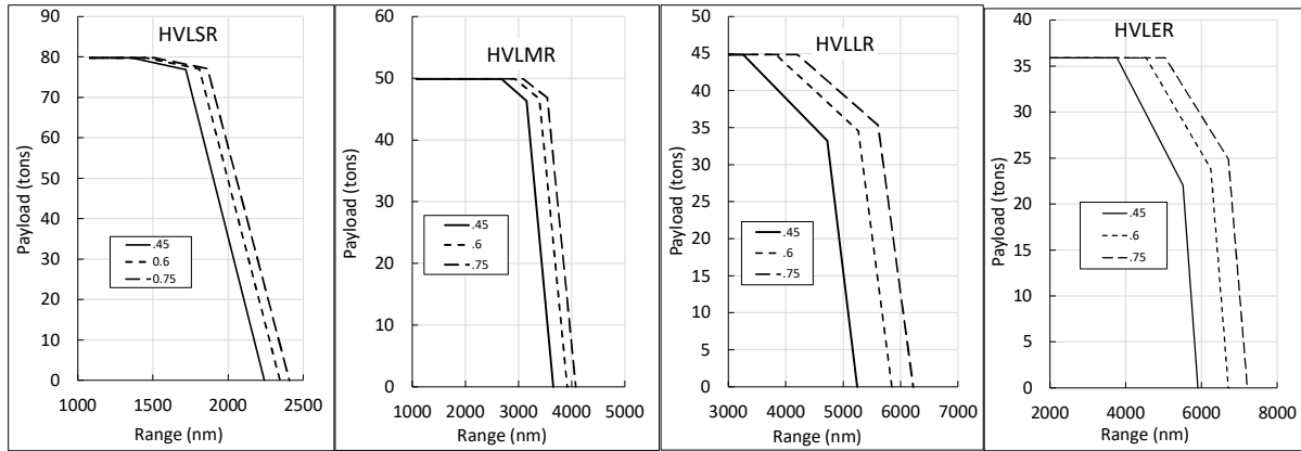
Figure 7 - Influence of \eta_{grav} on the payload range diagrams of the aircraft family
