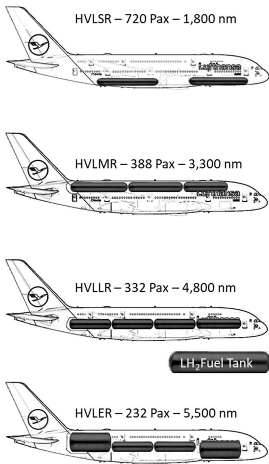
Figure 2 – Four airliner family concepts. Images courtesy (Lufthansa 2020) and modified by the authors.
