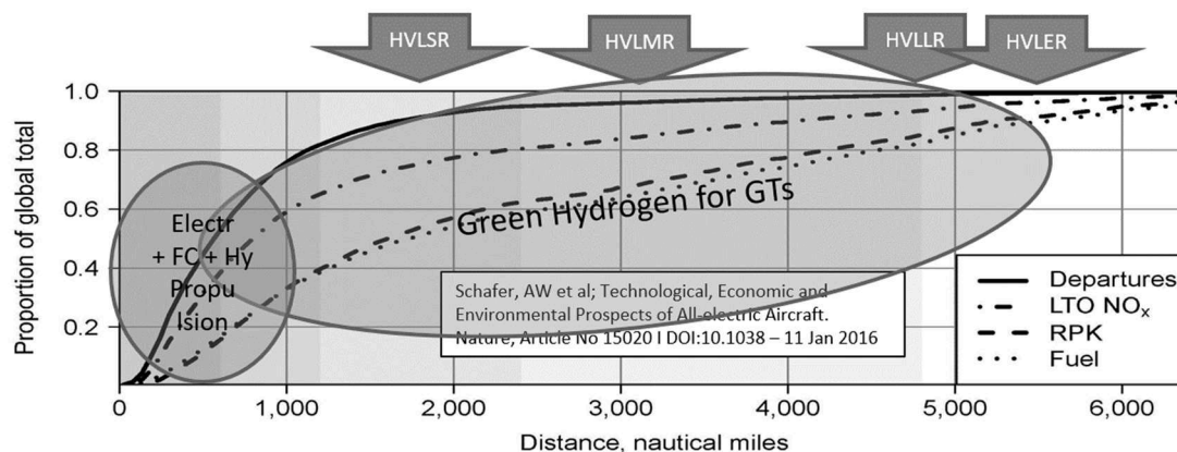
Figure 4 – HVLSR, HVLMR, HVLLR and HVLER capabilities with a baseline gravimetric efficiency of 0.45. (Schafer et al, 2016) annotated by the authors
