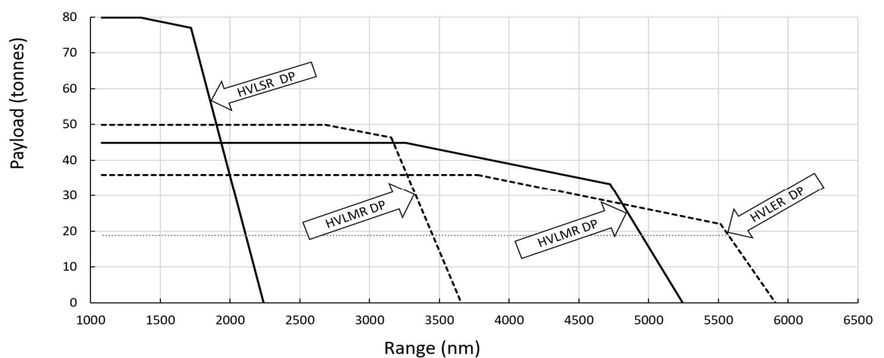
Figure 3 - Payload range diagrams for the aircraft family, for a gravimetric efficiency of 0.45 with the design points of figure 2 indicated.
