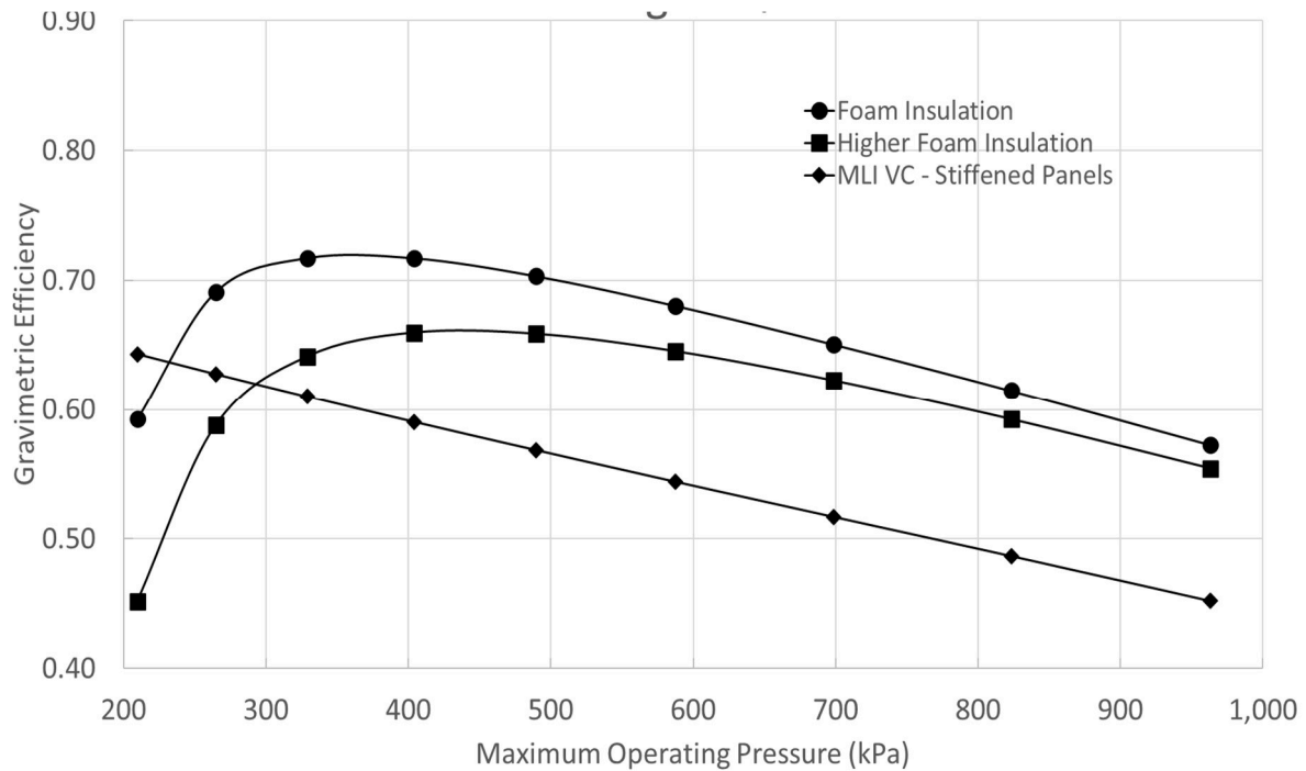
Figure 5 Gravimetric efficiency of tank options evaluated for a 100 m 3 tank. The tank is cylindrical with hemispherical ends, a diameter of 4m and a length of 9.3m.
