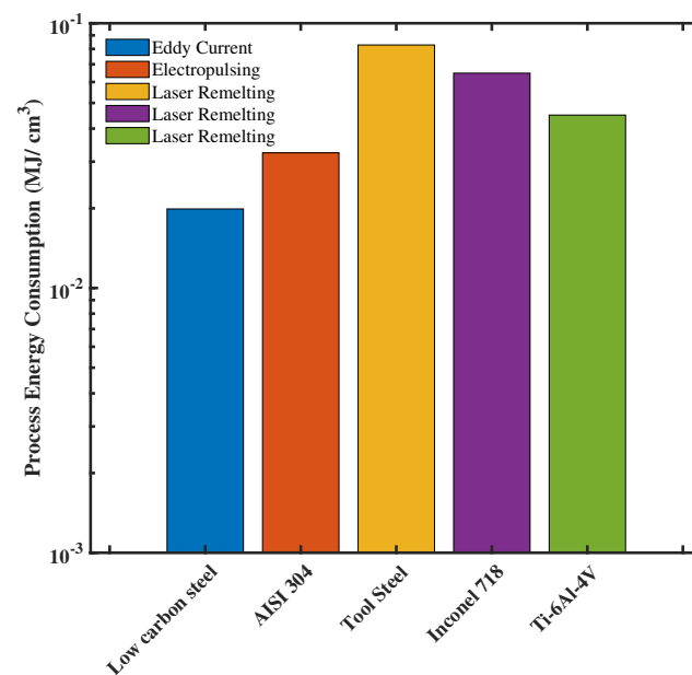
Figure 12. Comparison of energy consumption between different thermal processes for different materials.
