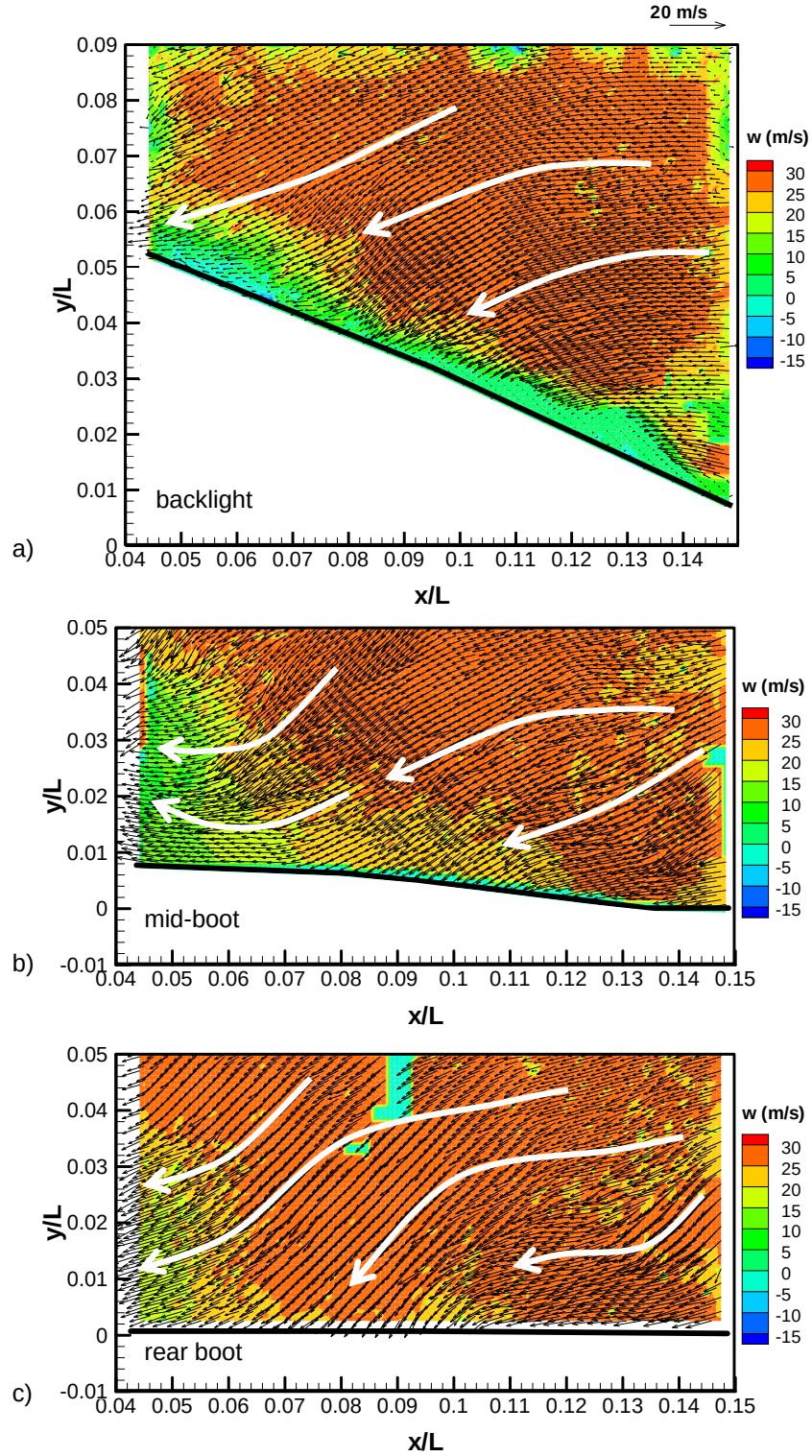
Figure 12 – 3D PIV data at V_\infty = 30 \text{ m/s} ( \text{Re} = 3.69 \times 10^6 ) a) backlight b) mid-boot c) rear boot
