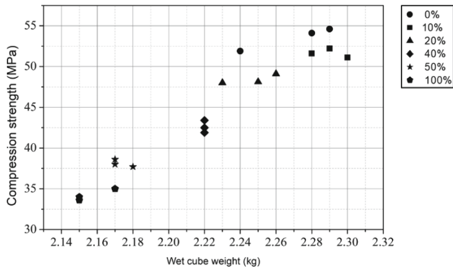
Fig. 2. Compression strength Vs wet cube weight (kg) for Wet cast
