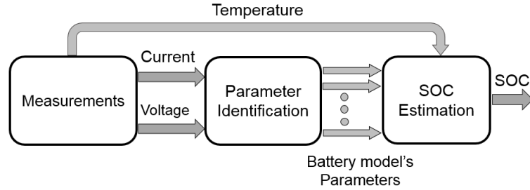
Figure 5: Battery measurement, identification and estimation in real-time
