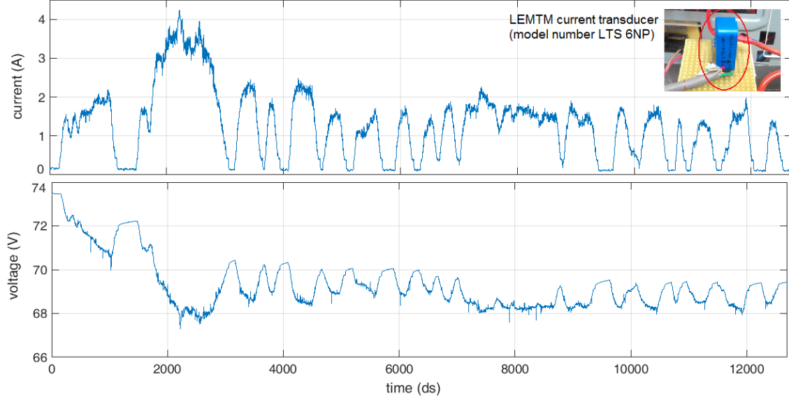
Figure 10: battery current and terminal voltage profiles for the first cycle
