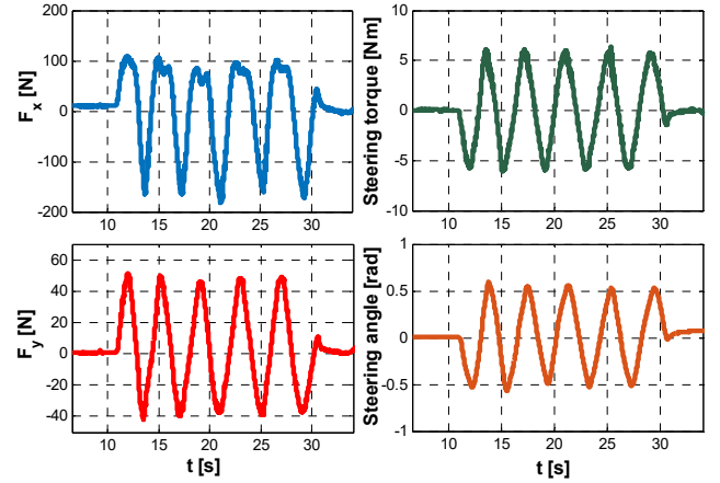
Fig. 6. Experimental data from the active steering task with right arm only at the 3 o'clock hand position.
