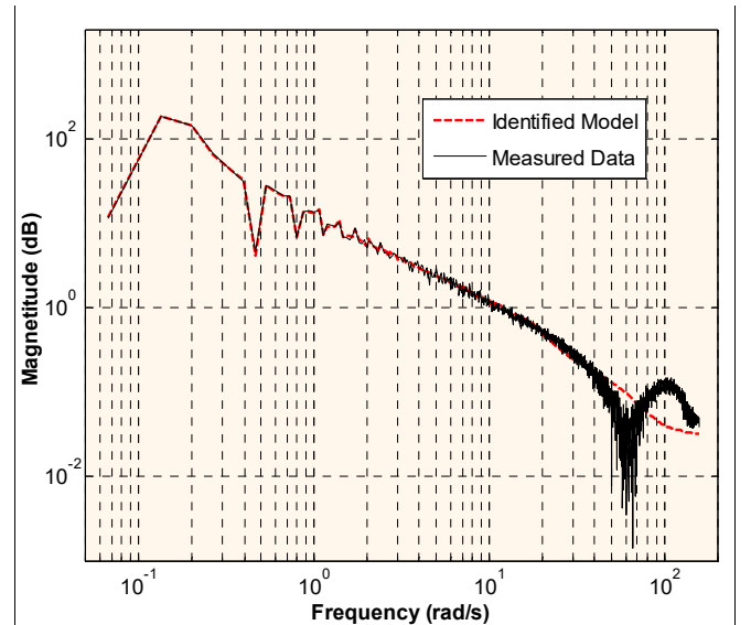
Fig. 7. Comparison of the amplitude curves of the data's and the models' frequency responses.
