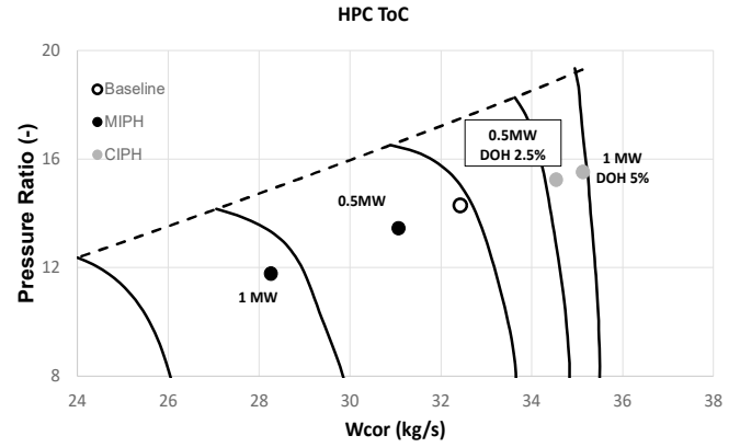
Figure 13: ToC HPC operating points for different DoH
