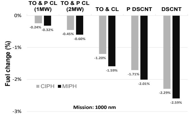
Figure 20: Fuel reduction for different PMS, 1000nm
