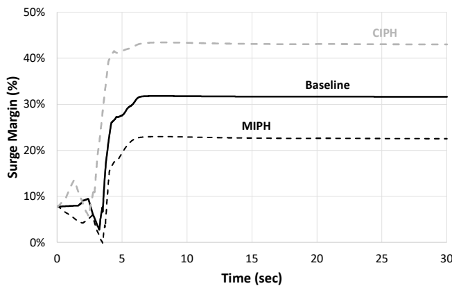
Figure 17 LPC surge margin change during slam acceleration
