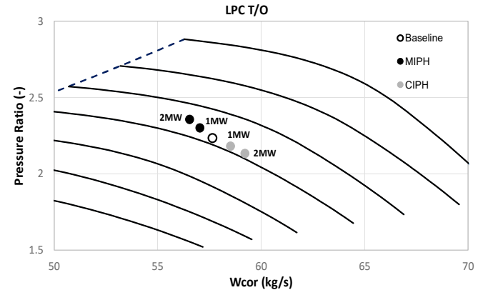
Figure 9: T/O LPC operating points for different DoH
