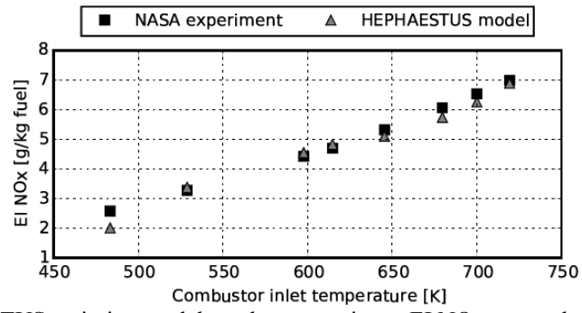
Figure 8 HEPHAESTUS emission model results comparison: EI NO x vs. combustor inlet temperature
