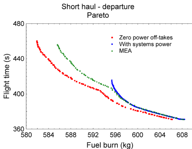
Fig. 8 Pareto fronts—departure, short haul
