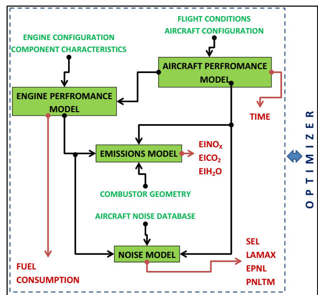
Fig. 4 Typical setup in GATAC for trajectory optimisation [25]
