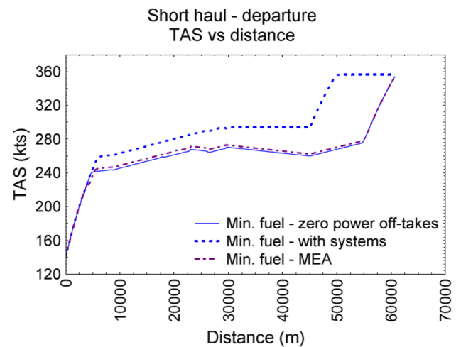
Fig. 10 True air speed vs distance—departure, short haul
