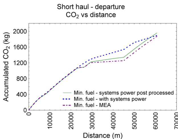
Fig. 13 Total CO 2 emissions vs distance—departure, short haul
