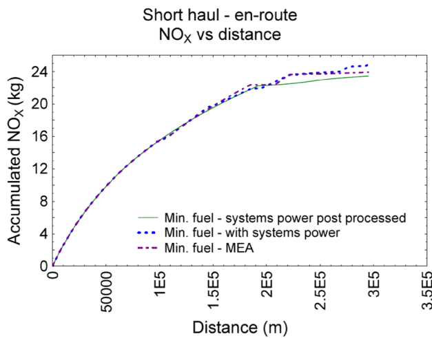
Fig. 18 Total \text{NO}_x emissions vs distance—en route, short haul
