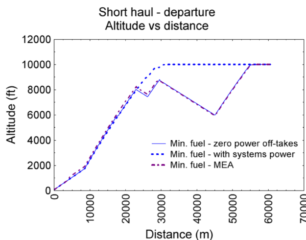
Fig. 9 Altitude vs distance—departure, short haul
