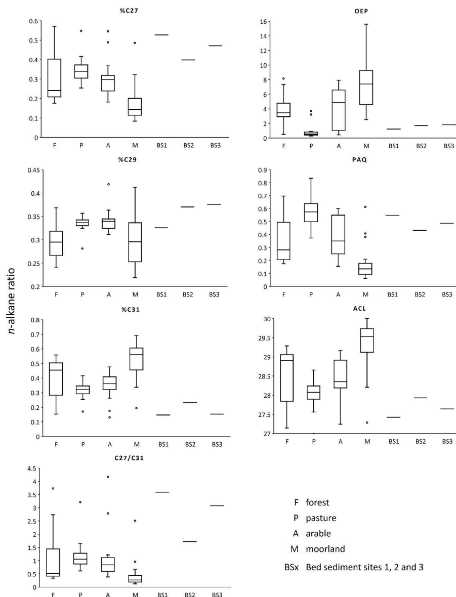
Fig. 4. Range of n-alkanes ratios C27/C31, %C27, %C29, %C31, OEP, PAQ and ACL from forest, pasture, arable and moorland land uses and streambed sediment sources. The box is extended from the 25–75 percentiles, the line is plotted at the median and whiskers show the maximum to minimum range excluding outliers (dots).
