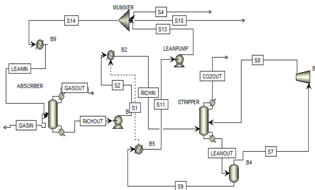
Figure 4. Vapor recompression modification [11].
