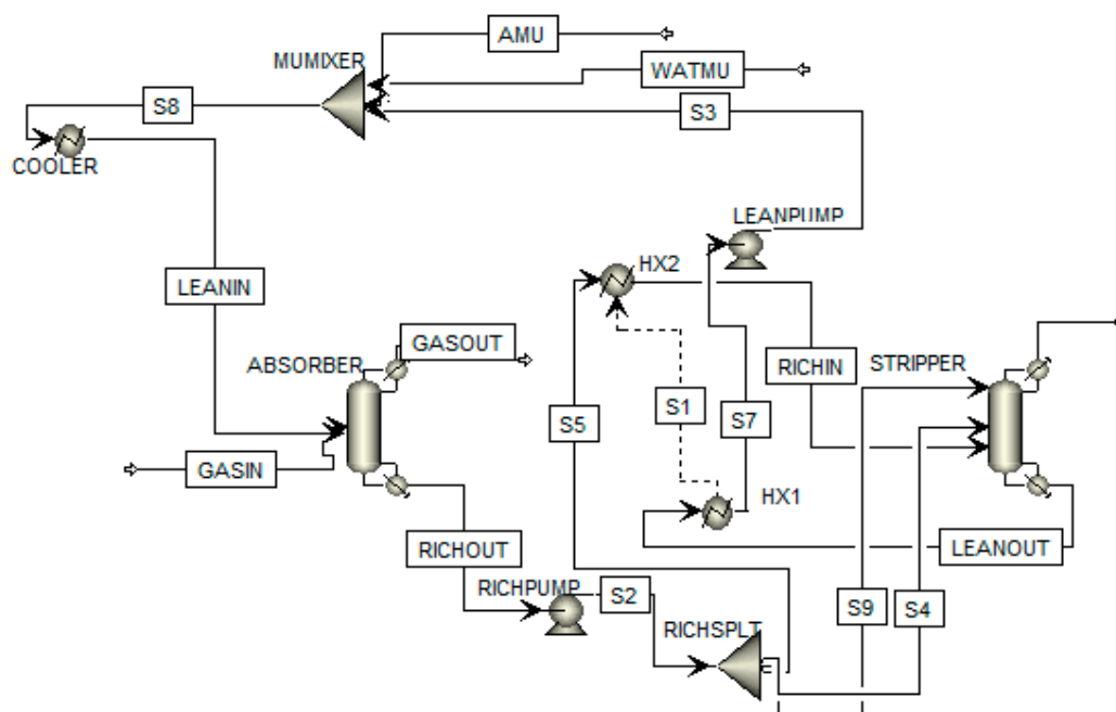
Figure 3. Rich split modification [11].
