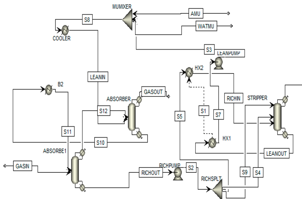
Figure 5. Rich split with intercooling configuration.
