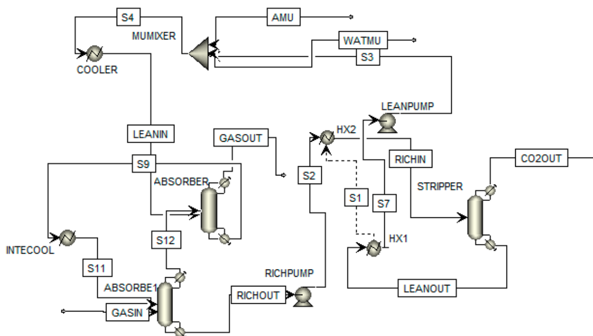
Figure 1. Intercooling Configuration [11].
