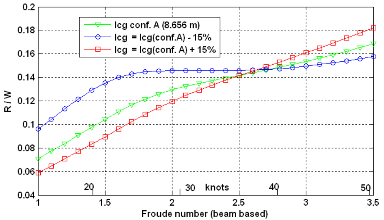
Figure 7: Influence of the longitudinal position of CG considering the Resistance-to-Weight ratio
