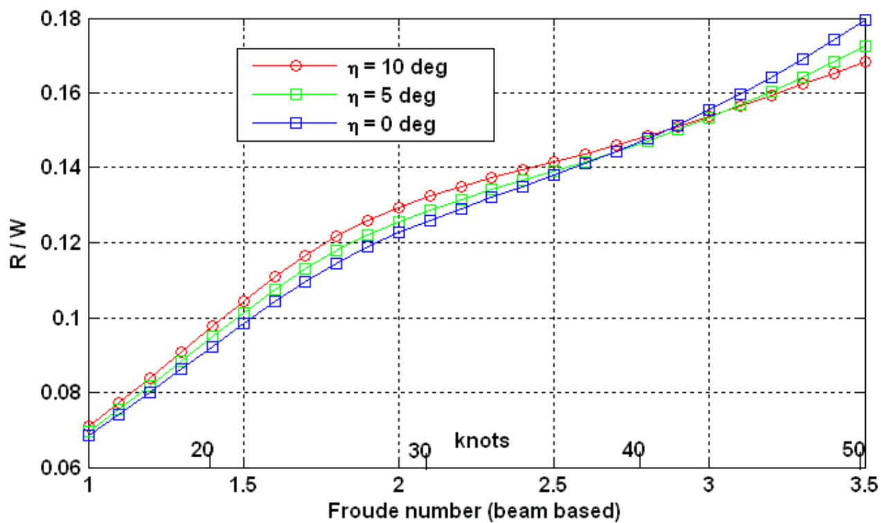
Figure 6: influence of \eta considering the Resistance-to-Weight ratio
