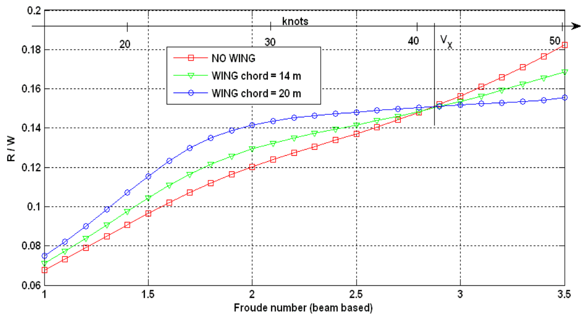
Figure 5: influence of the wing area considering the Resistance-to-Weight ratio
