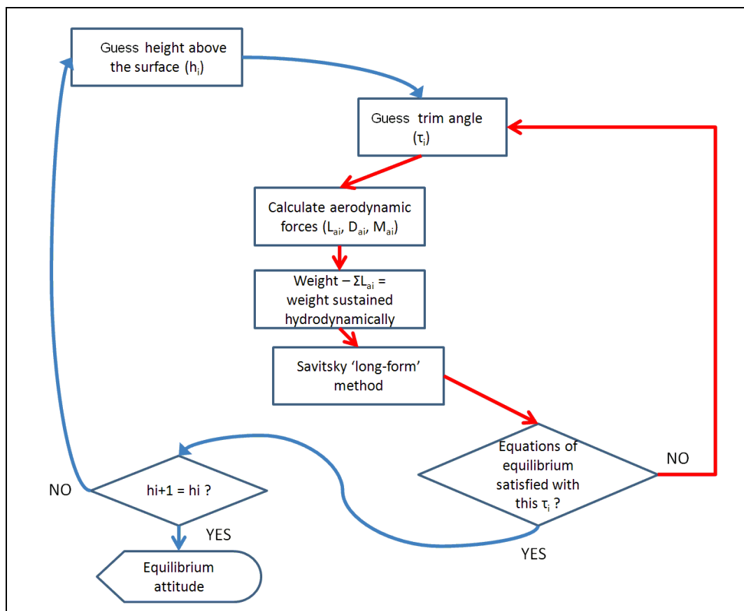
Figure 3: flow chart of the method to find the equilibrium attitude of the HV
