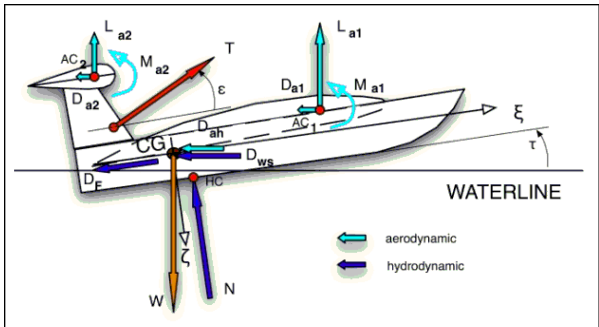
Figure 2: forces and moments acting on the hybrid vehicle
