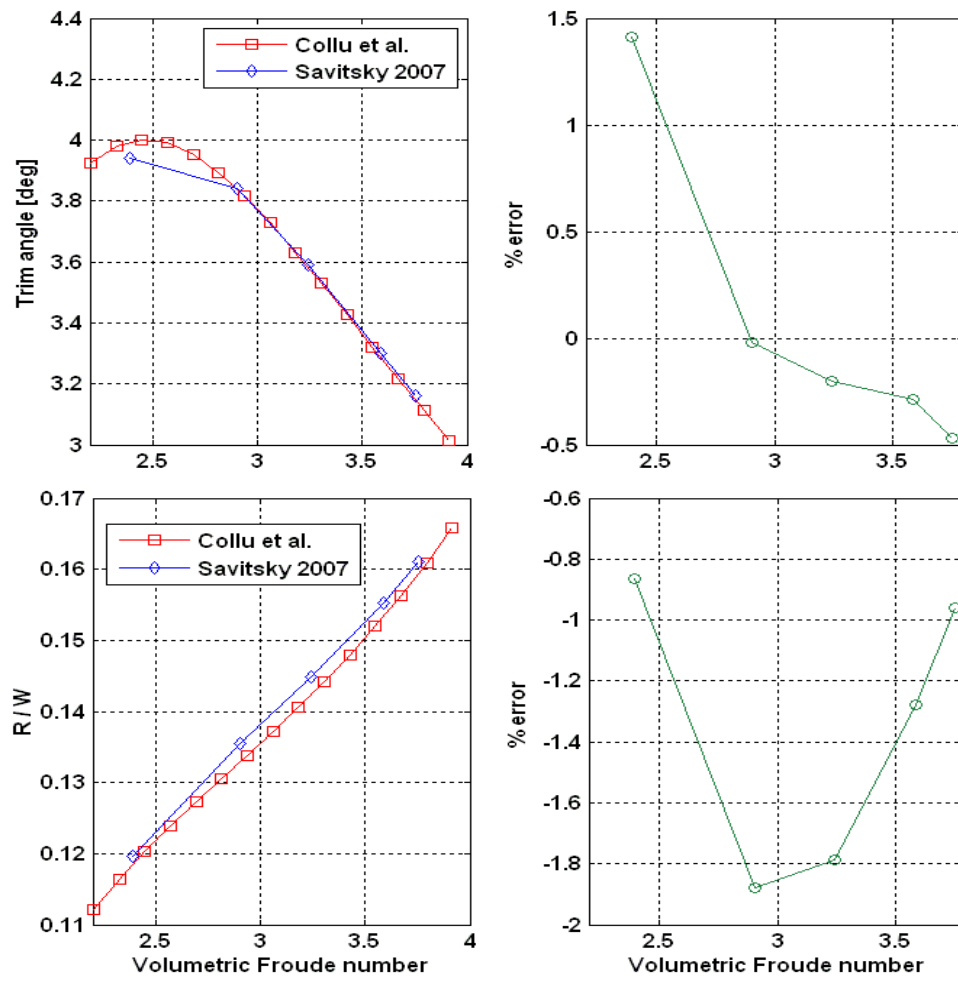
Figure 4: Savitsky 2007 (15) vs. Collu et al. – Trim angle and Resistance-to-Weight ratio
