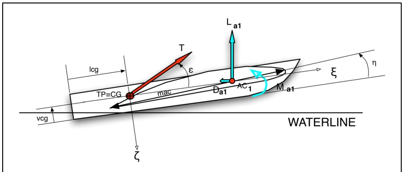
Figure 1: characteristics of the analyzed configurations
