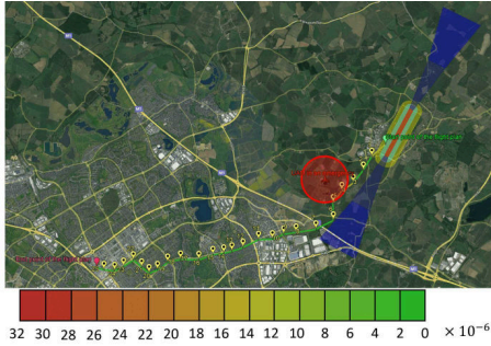
Fig. 11. Risk of flight plan to the air.
