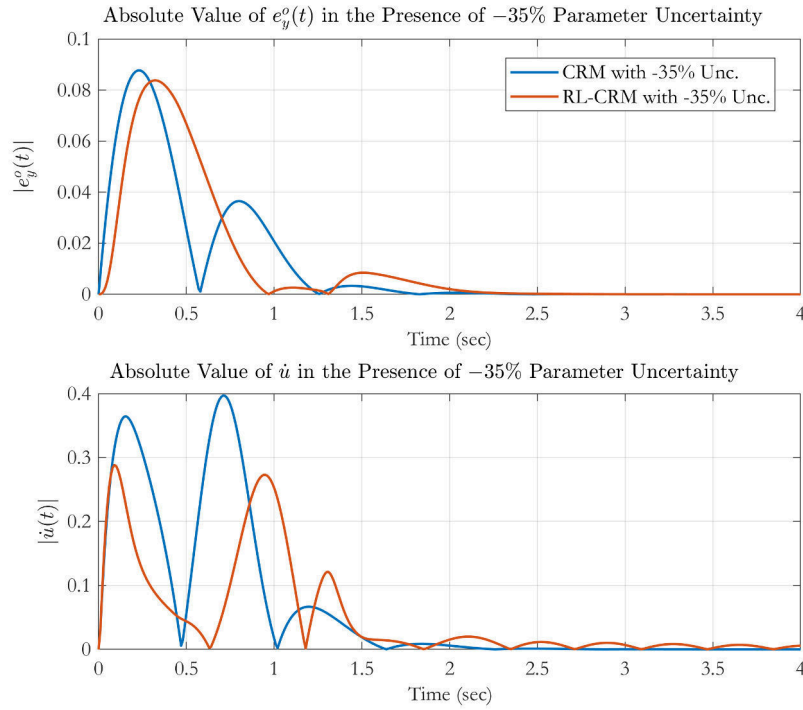
FIGURE 11 Comparison of |e_y^o(t)| and |\dot{u}(t)| time history of the CRM and RL-CRM systems in the presence of -35\% parametric uncertainty.
