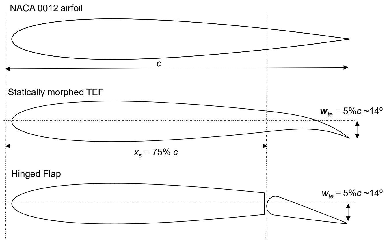
Figure 2. Mid-span slices showing the configurations studied and their dimensions.
