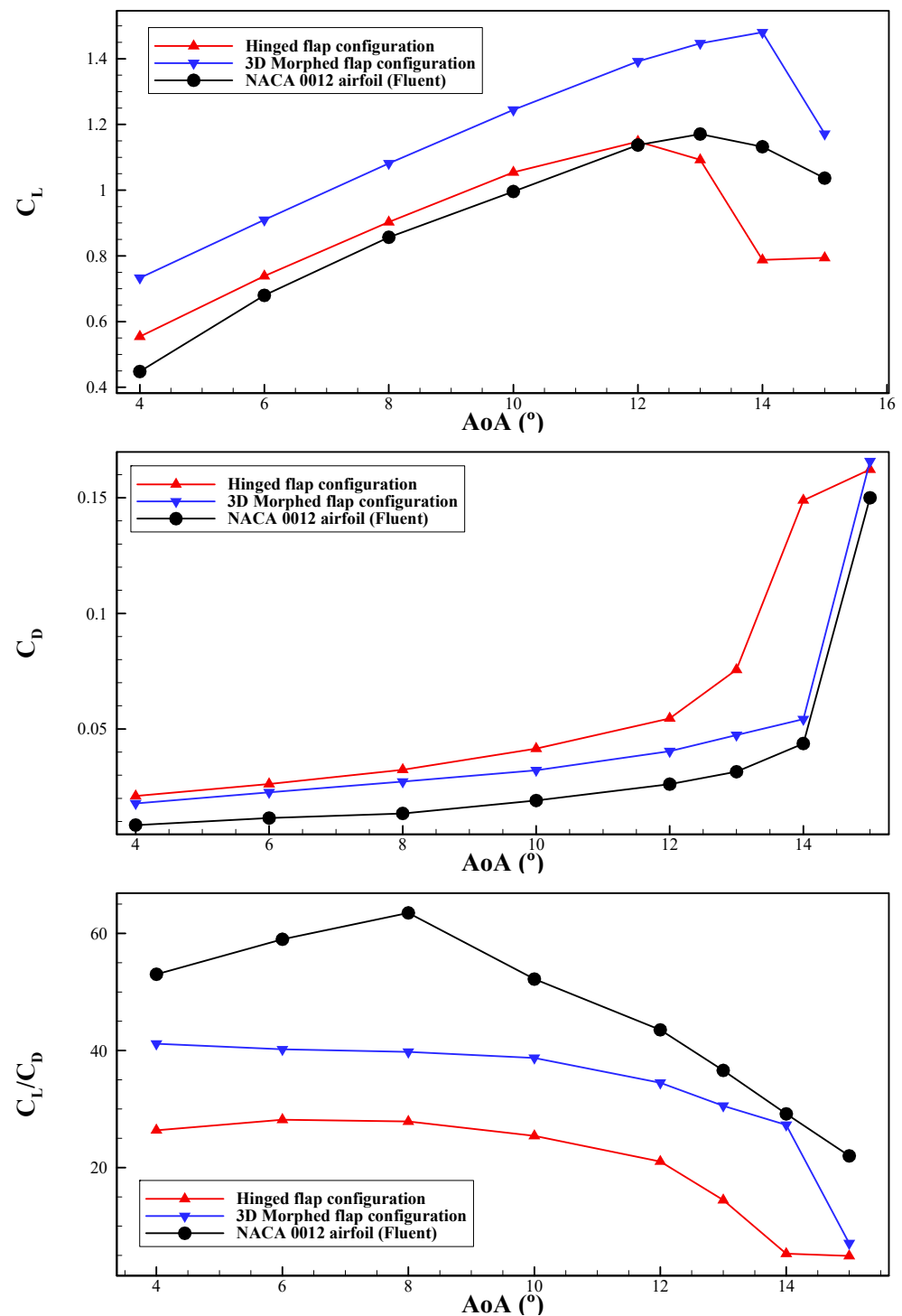
Figure 7. Comparative results for C_L and C_D and the aerodynamic efficiency ( C_L/C_D ) for the baseline NACA 0012 wing, the wing equipped with a morphed flap and the one with a hinged flap in addition to the 2D prediction of an airfoil with a morphed TEF.
