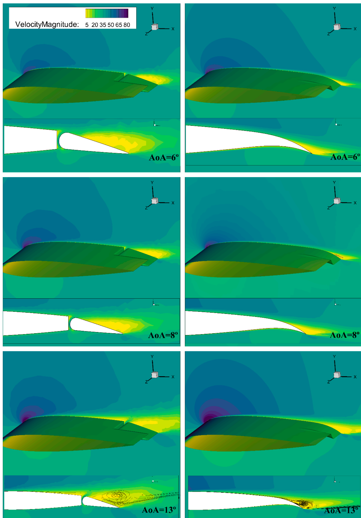
Figure 8. Velocity contours comparison at mid-span between the wing with the hinged and a morphed TEF at AoA = 6°, 8° and 13°. The close-ups show the side view at mid-span for both configurations.
