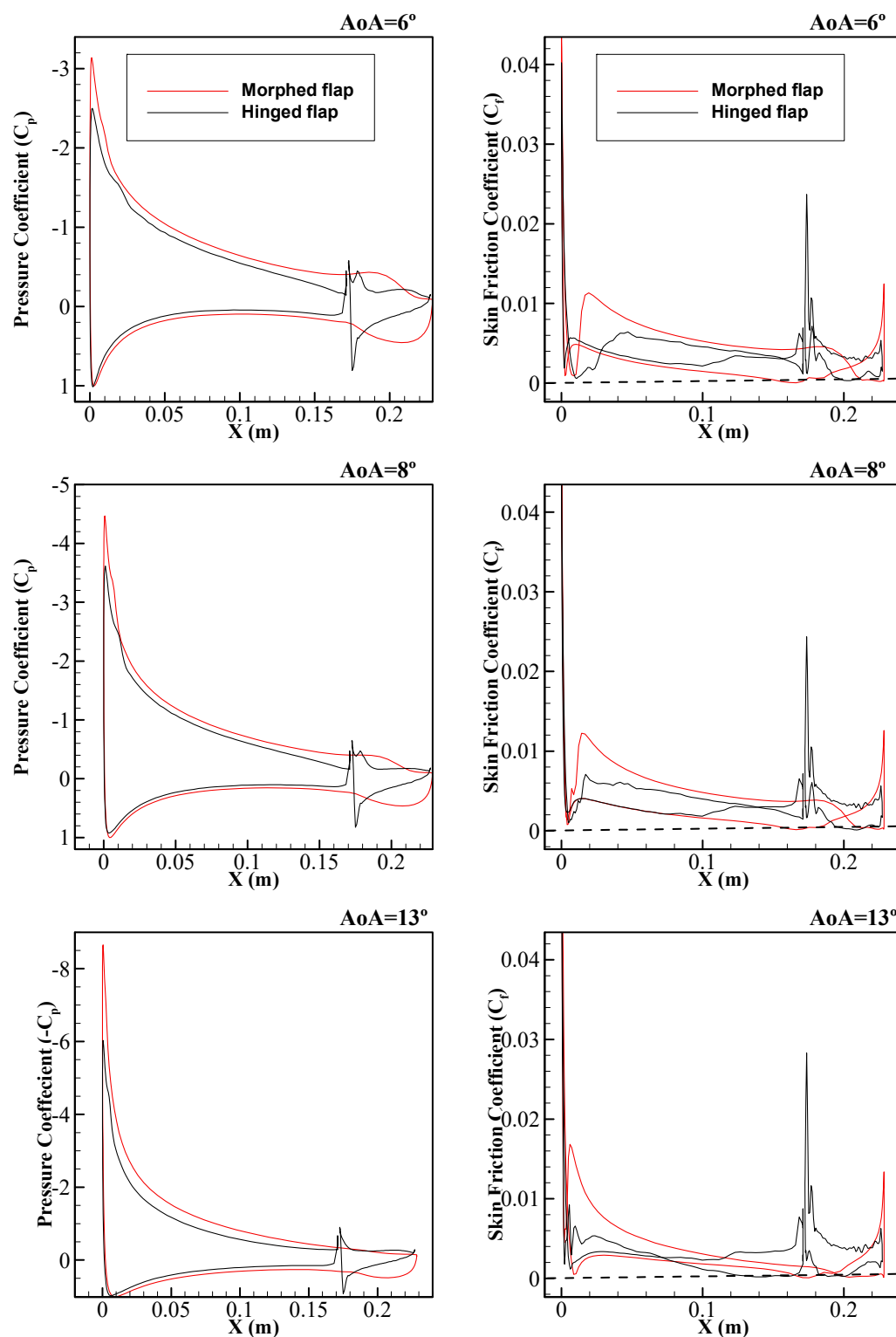
Figure 10. C_p and C_f comparison between the wing with a morphing TEF and seamless transition and the wing with a hinged flap, mid-span location at AoA = 6°, 8° and 13° from top to bottom.
