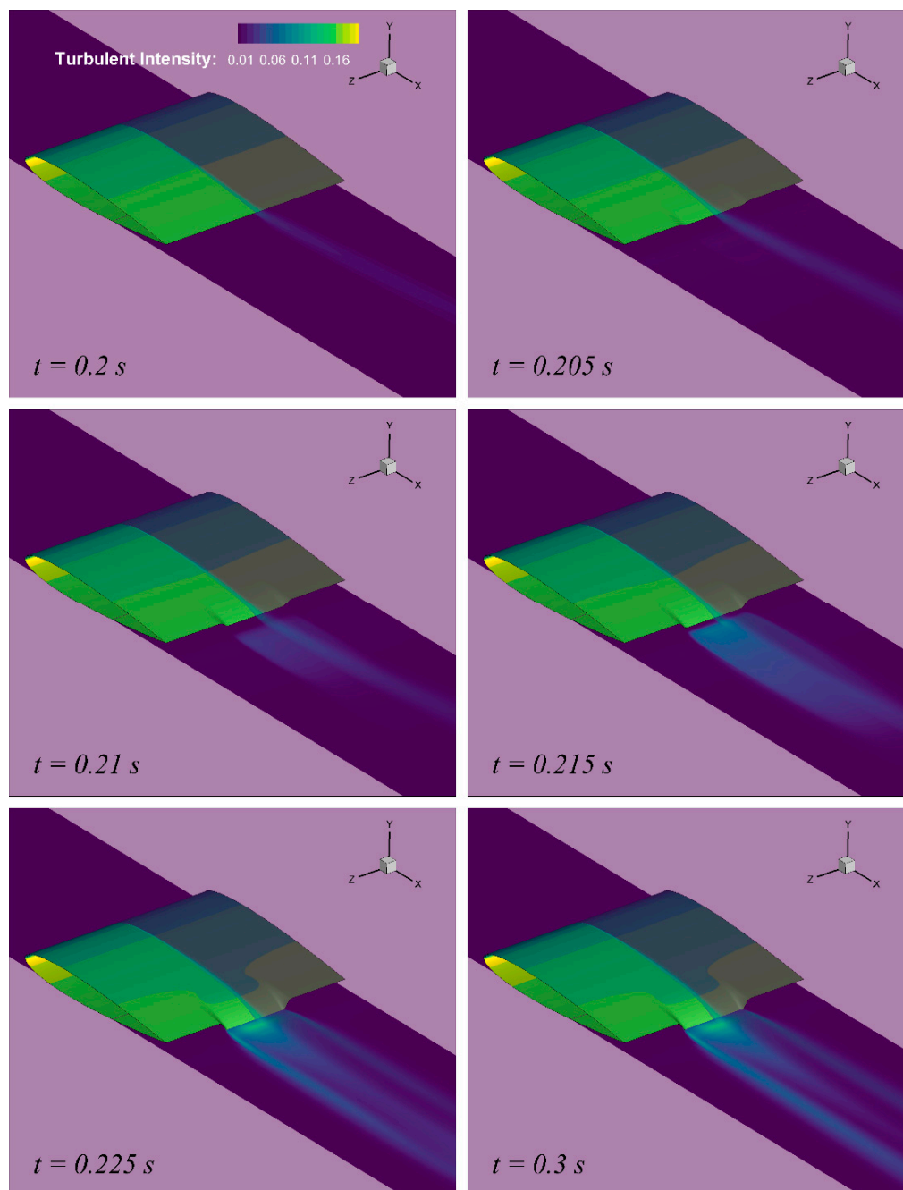
Figure 17. Instantaneous turbulent intensity contours placed at three stations and six time instances illustrating the dynamic morphing process of a 3D wing with seamless side-edge transitions at \text{AoA} = 6^\circ and a morphing frequency of 8 Hz.
