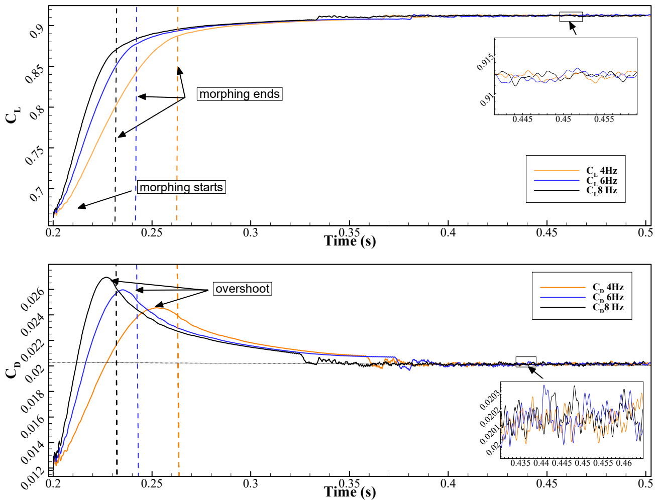
Figure 13. Time history of C_L and C_D for the dynamically morphing TEF of the wing with side transition at AoA = 6^\circ for three morphing frequencies.
