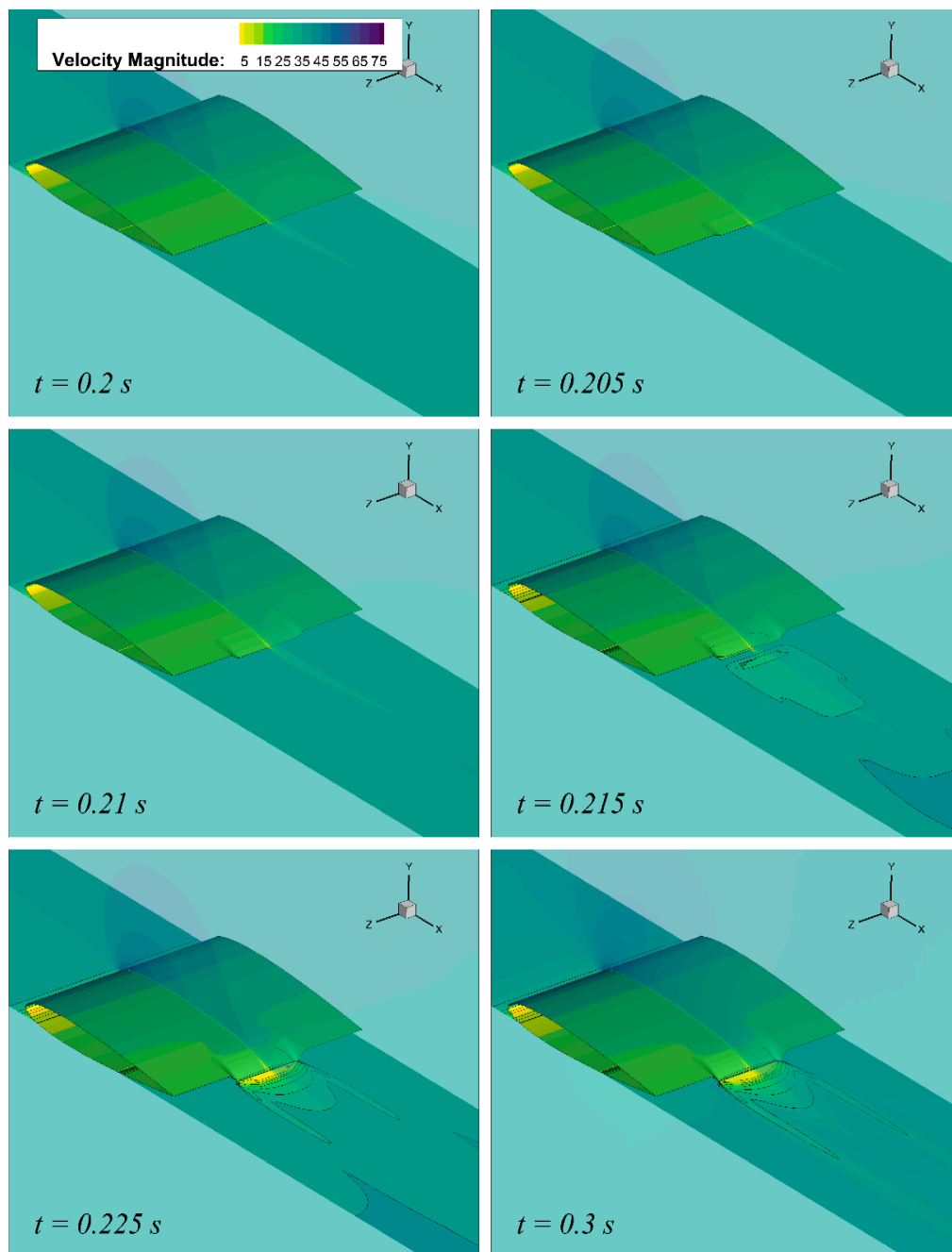
Figure 16. Instantaneous velocity contours placed at three stations at six time instances illustrating the dynamic morphing process of a 3D wing with seamless side-edge transitions at \text{AoA} = 6^\circ and a morphing frequency of 8 Hz.
