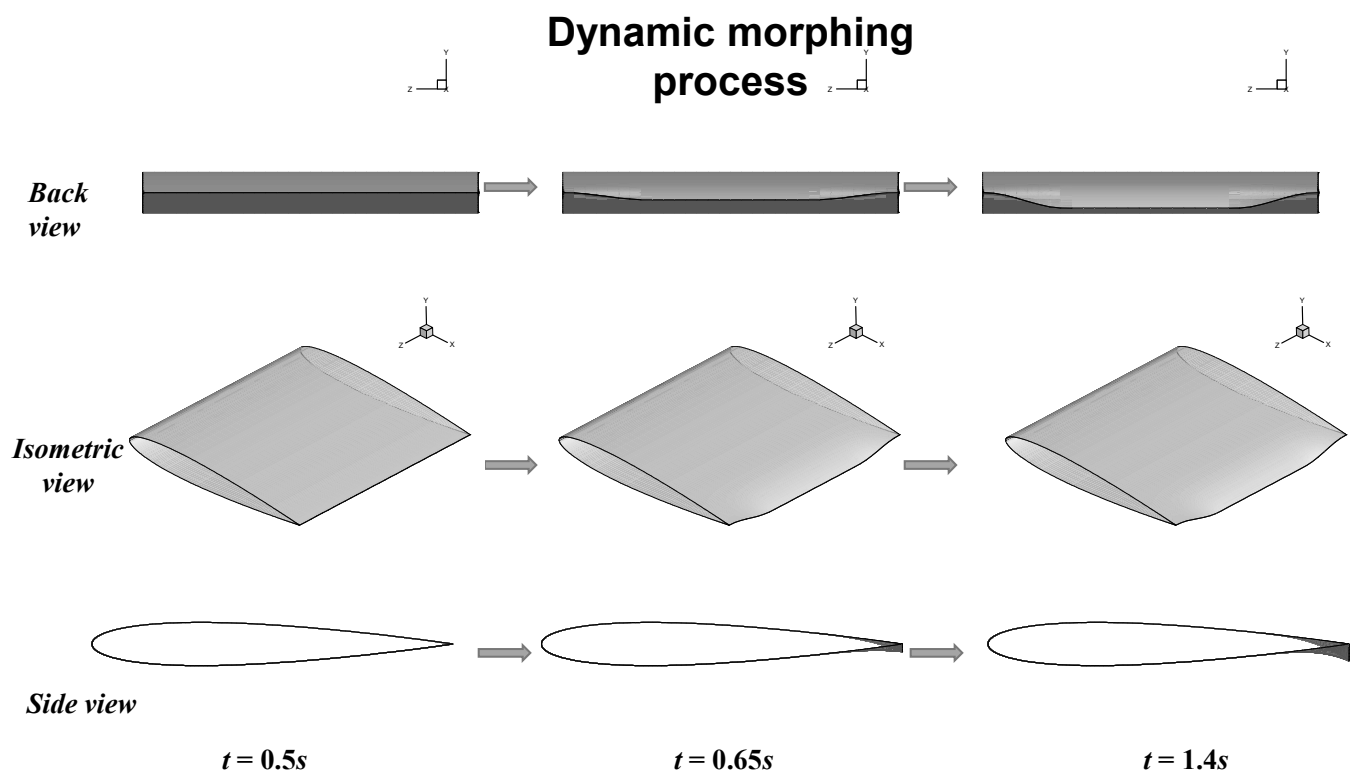
Figure 1. Illustration showing the dynamic morphing process driven by the modified unsteady parametrization method.
