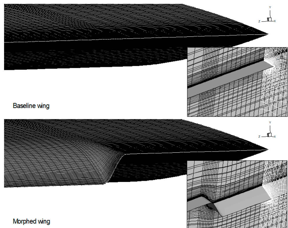
Figure 5. Direct comparison between the baseline un-deformed mesh ( upper ) and the mesh after the TEF deformation ( lower ).
