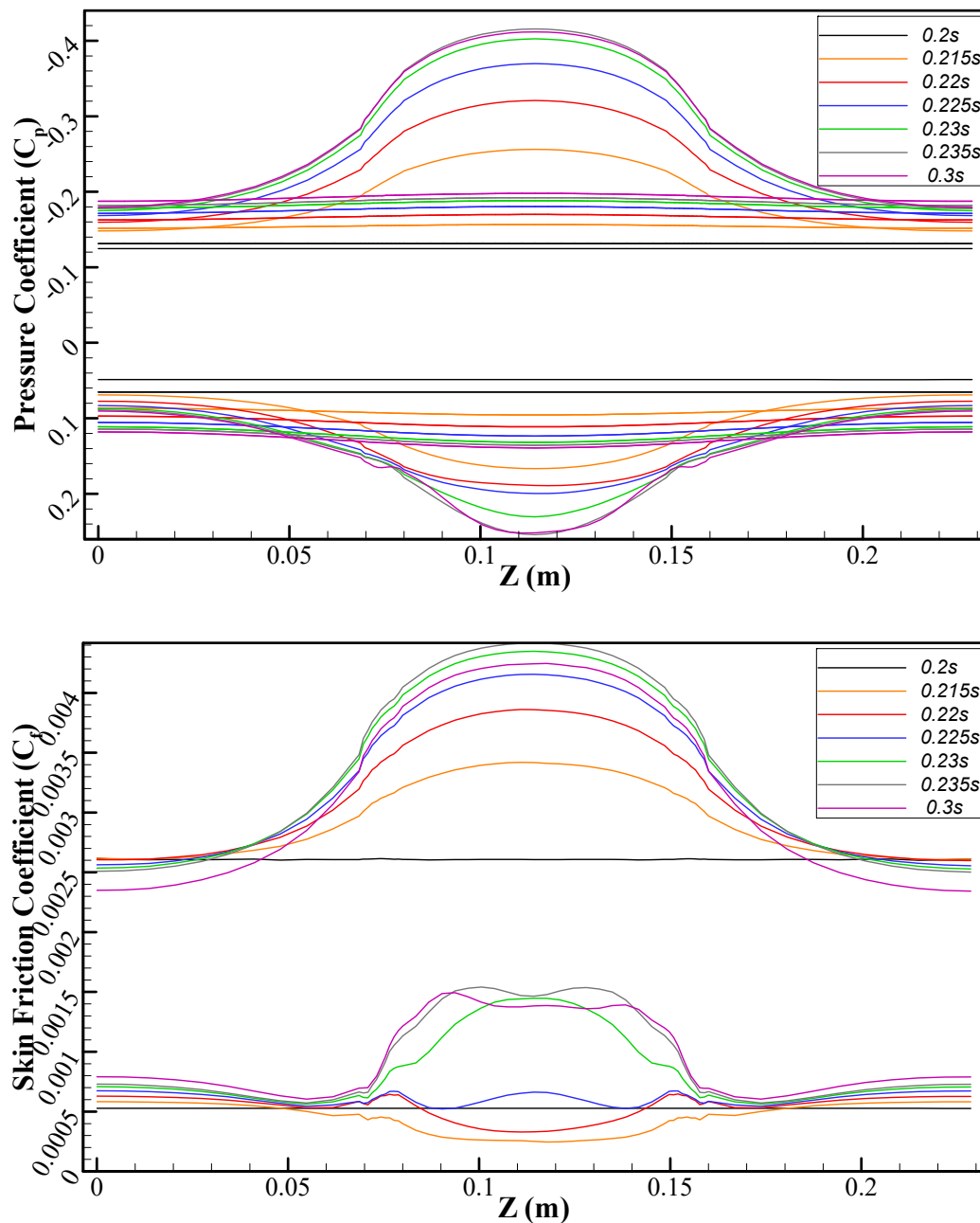
Figure 15. Instantaneous C_p (top) and C_f (bottom) for the dynamically morphing TEF at \text{AoA} = 6^\circ on a slice at x = 0.8c .
