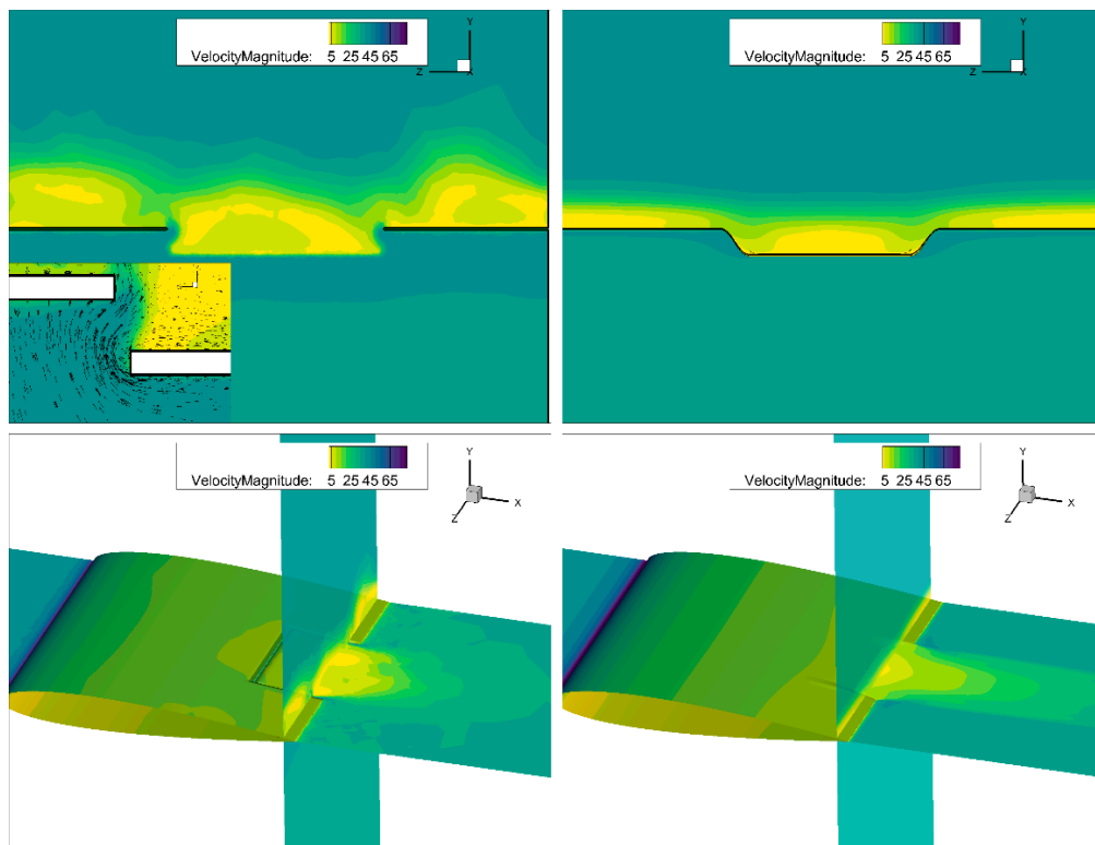
Figure 9. Top: Velocity contours and vectors of the wing with a morphed TEF flap ( top right ) compared with the one with a hinged flap ( top left ) on a plane placed at x = 0.99c at \text{AoA} = 13^\circ . Bottom: wake flow structure visualisation by means of velocity contours with a slice at y = 0 and x = 0.95c .
