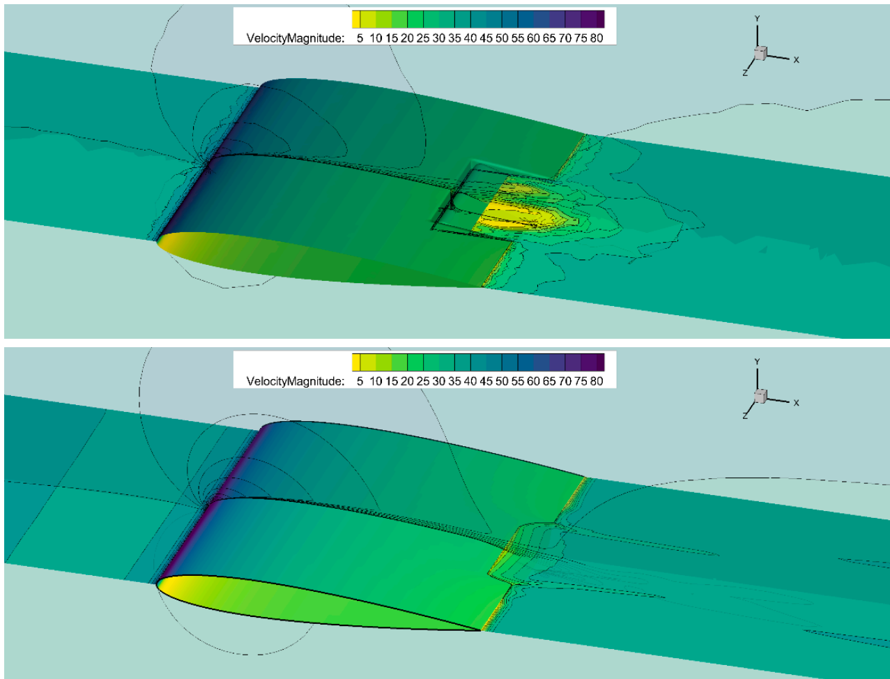
Figure 12. Visualization of flow separation by means of velocity contours with a slice at y = 0 and x = 0.95c comparing the wing with a morphing TEF and seamless transition ( bottom ) and the wing with a hinged flap ( top ).
