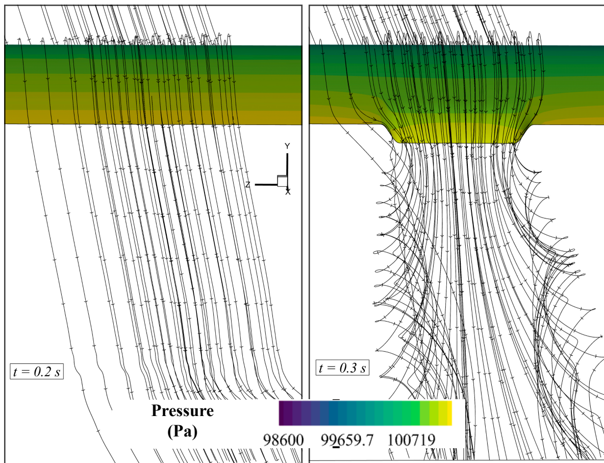
Figure 18. Streamlines and surface pressure contours illustrating the 3D effect induced by the dynamic morphing process of a 3D wing with seamless side-edge transitions, in comparison to a baseline configuration, before morphing starts ( \text{AoA} = 6^\circ , morphing frequency = 8 Hz).
