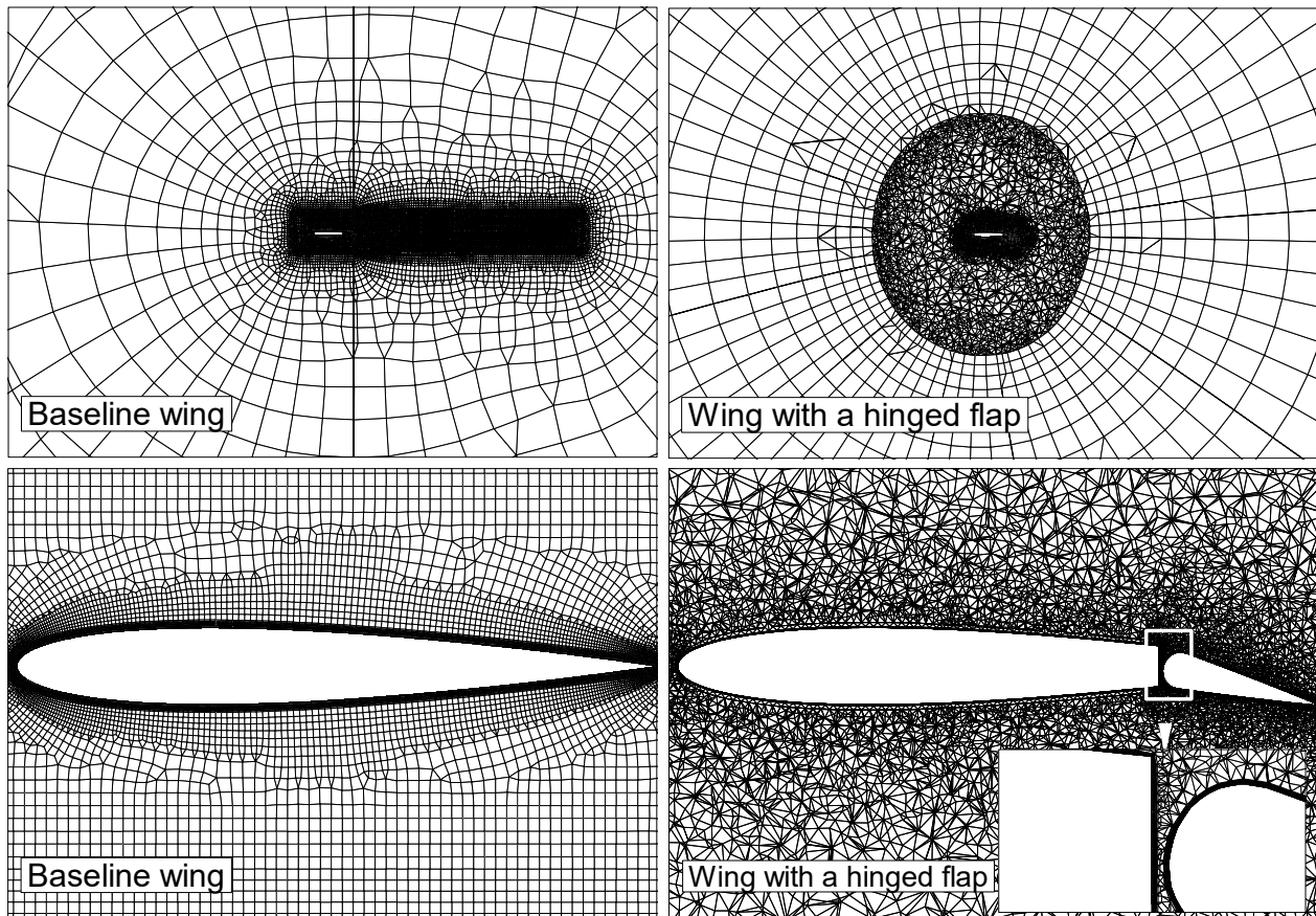
Figure 4. Computational domains used studies with close-up of the baseline NACA0012 wing and hinged flap wing.
