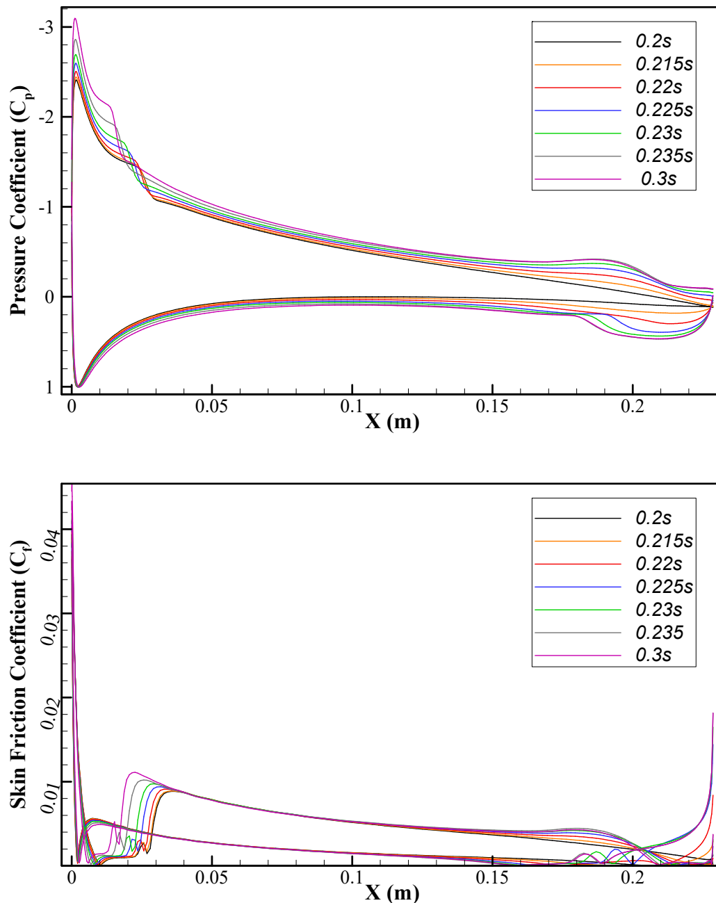
Figure 14. Instantaneous C_p (top) and C_f (bottom) distributions for the dynamically morphing TEF at \text{AoA} = 6^\circ at a mid-span slice ( z = 0.5S ).
