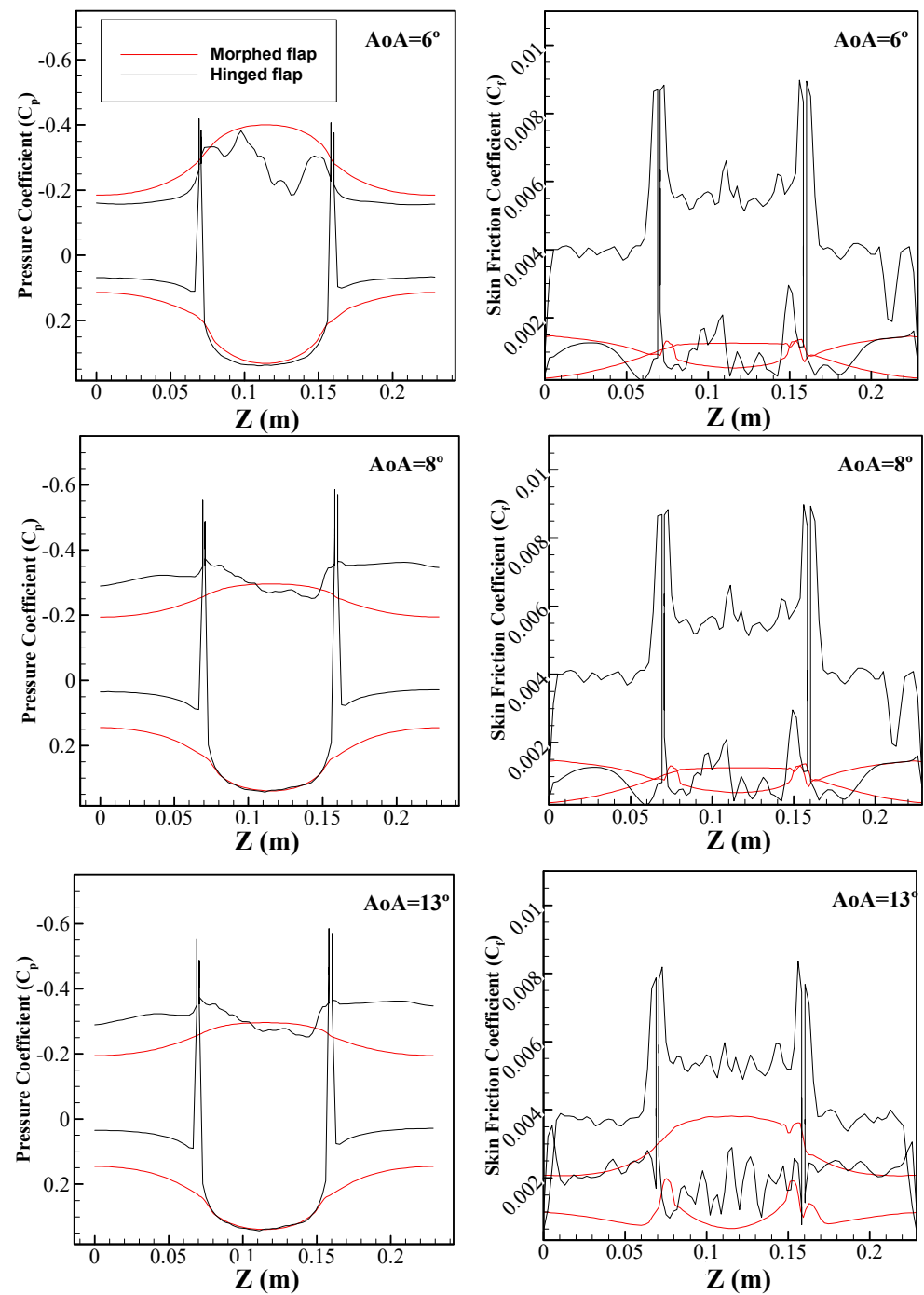
Figure 11. C_p and C_f comparison between the wing with a morphing TEF and seamless transition and the wing with a hinged flap, x = 0.8c location at AoA = 6°, 8° and 13° from top to bottom.
