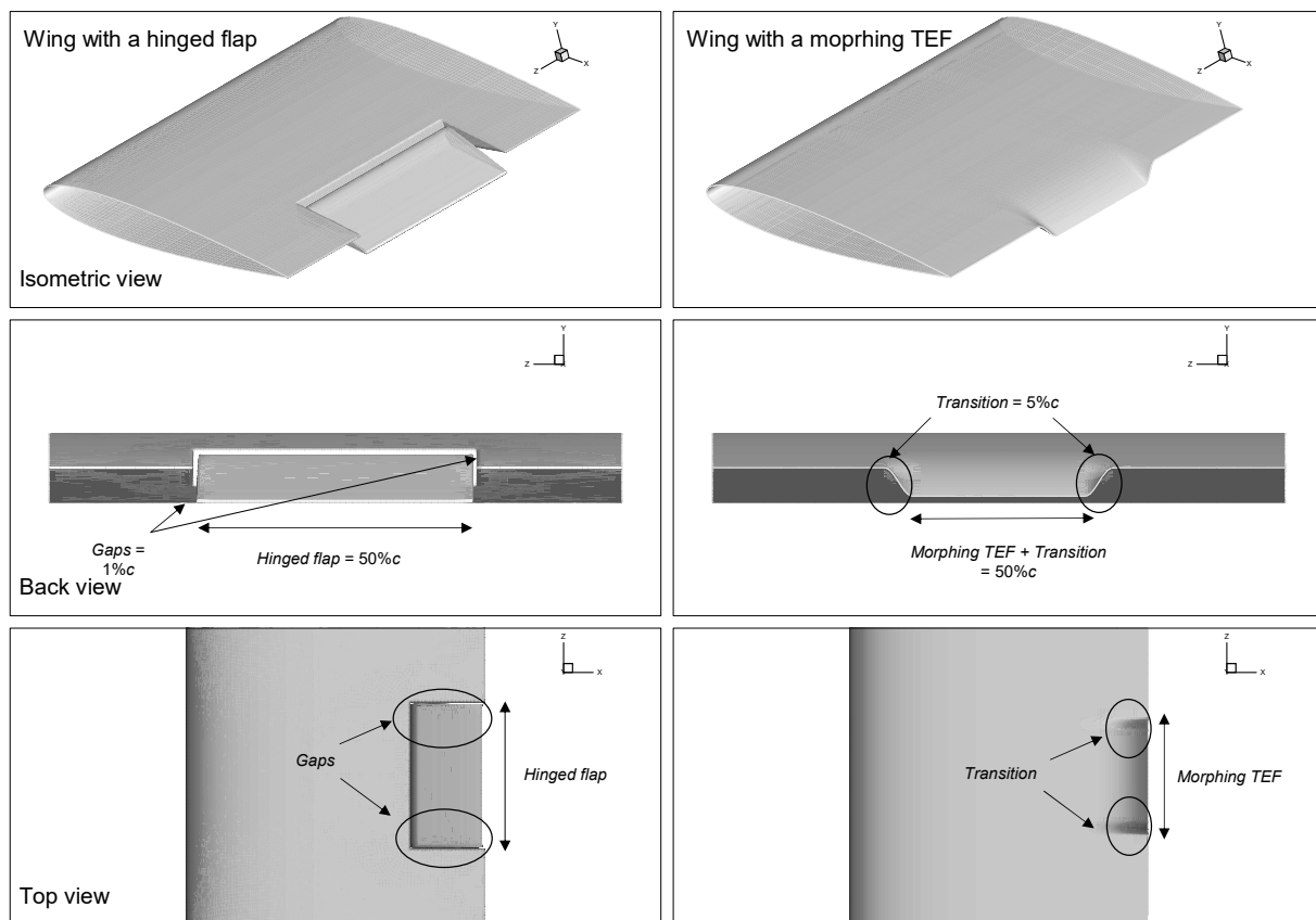
Figure 3. 3D models of the statically morphed wing and the hinged flap wing from various views.
