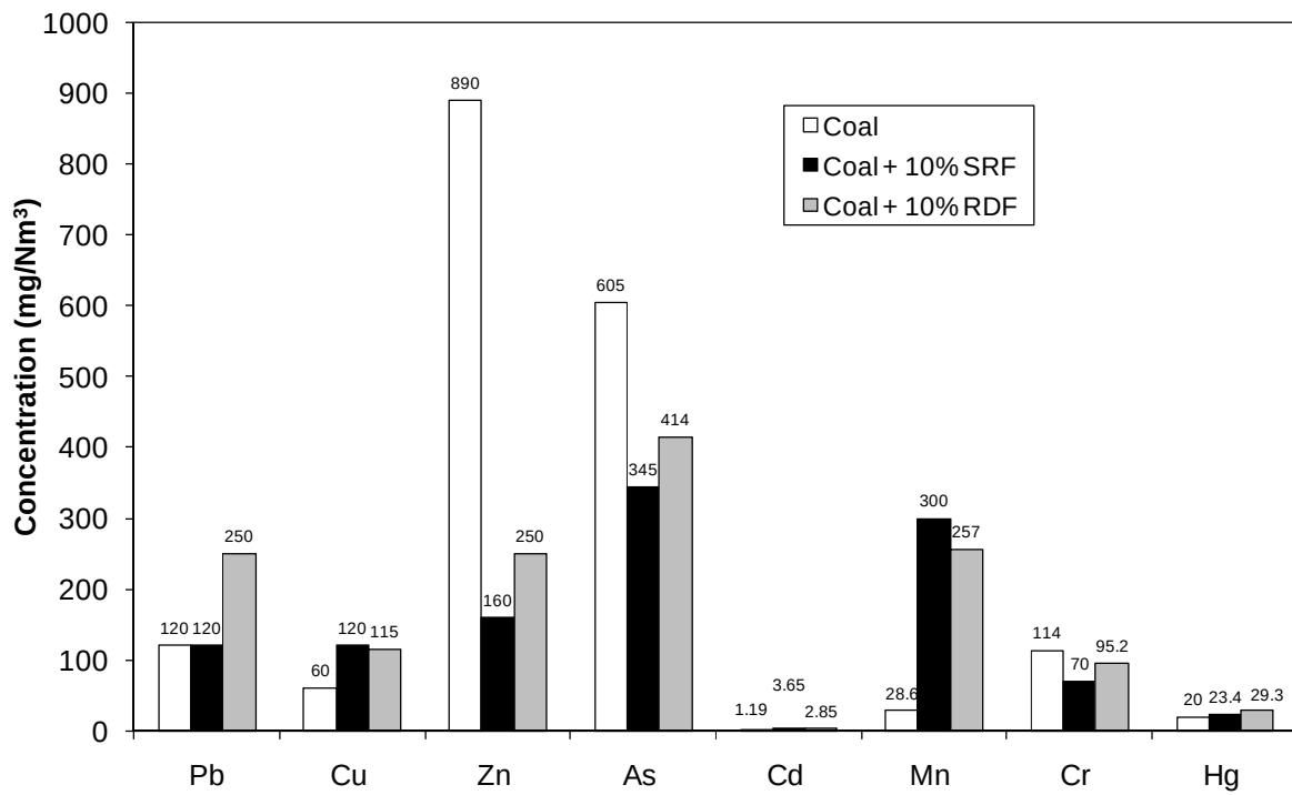
Figure 2. Metals concentration in flue gas samples obtained during the combustion of coal, (coal + 10% SRF) and (coal + 10% RDF) fuels
