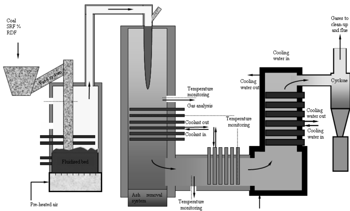
Figure 1. Schematic diagram of fluidized bed combustor
