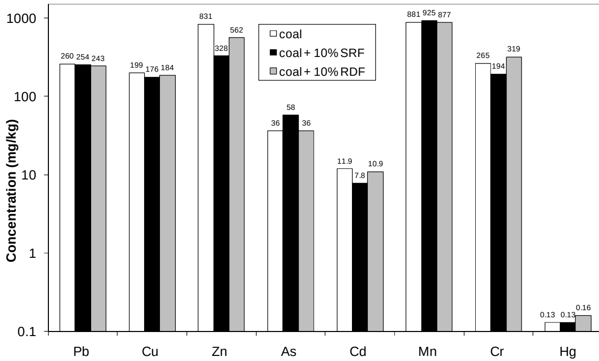
Figure 4. Metal concentrations in the fly ash samples obtained after combustion of fuels
