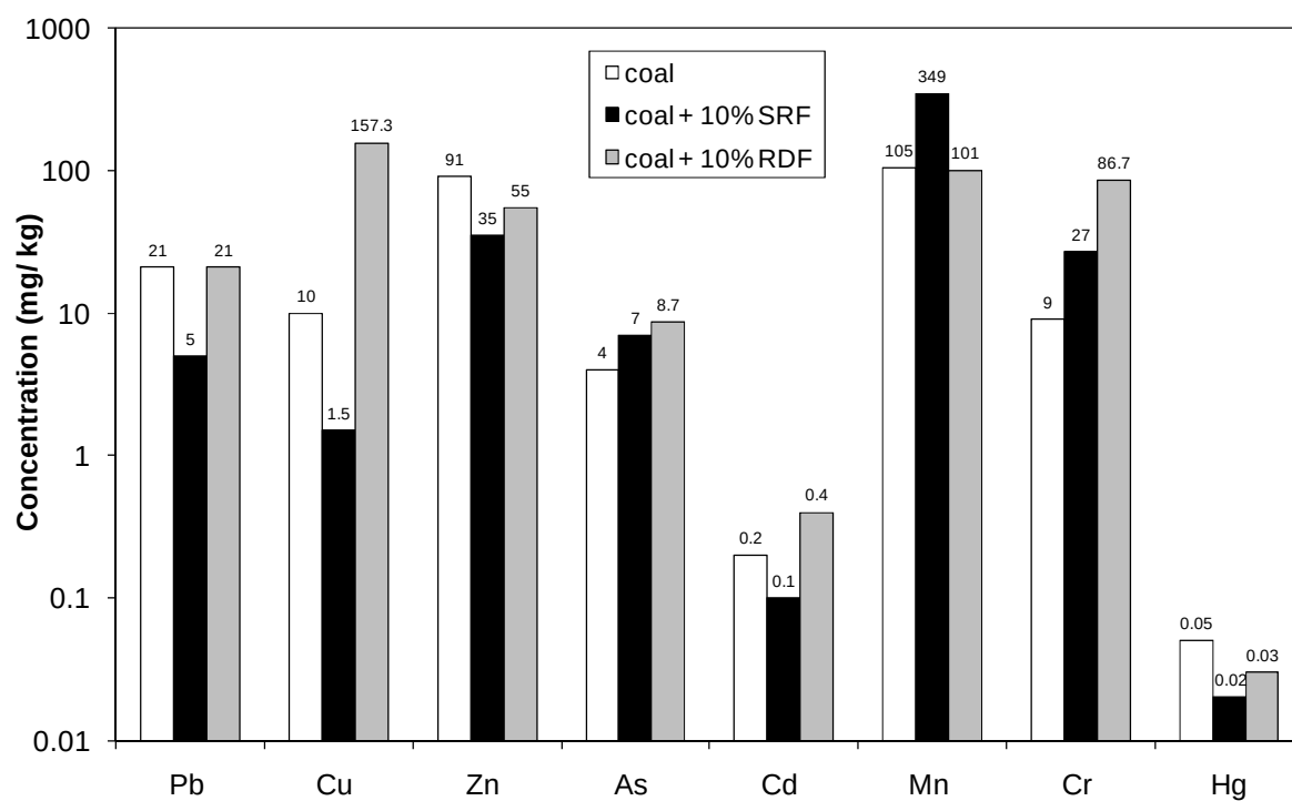
Figure 3. Metal concentrations in the bottom ash samples obtained after combustion of fuels
