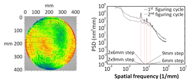
Figure 2. Topography map (left), averaged directional PSD plots across 400mm diameter ULE glass surface (Courtesy Castelli) (right).
