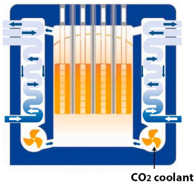
Fig. 1. Schematic Advanced Gas-cooled Reactor (AGR).
