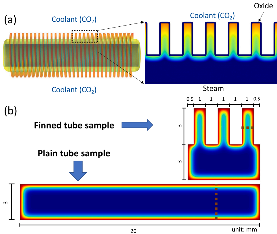
Fig. 2. (a): Illustration of the experimental finned and plain tube sample geometry; (b): dimensions of the finned tube and plain tube samples with illustrative carbon concentration fields; samples are profiled across the fin tip and the tube base as illustrated in dashed brown lines.
