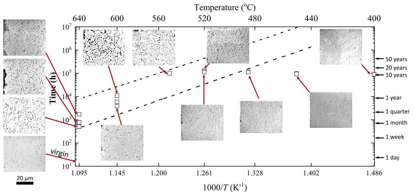
Fig. 5. Typical ion-induced secondary electron images collected at the spinel/substrate interface, for samples exposed at different combinations of temperature and time; the bottom left image shows the virgin condition (prior to CO 2 exposure). To guide the eye, predicted time of carbon saturation with \eta_{C}^{crit} = 0.2 and \eta_{C}^{crit} = 0.9 (using the Arrhenius fit of both \alpha_s/V_m and \zeta for a 1D domain corresponding to the fin width, considering oxidation kinetics, see Section 4) are shown as the dashed dot line and the dashed line, respectively.
