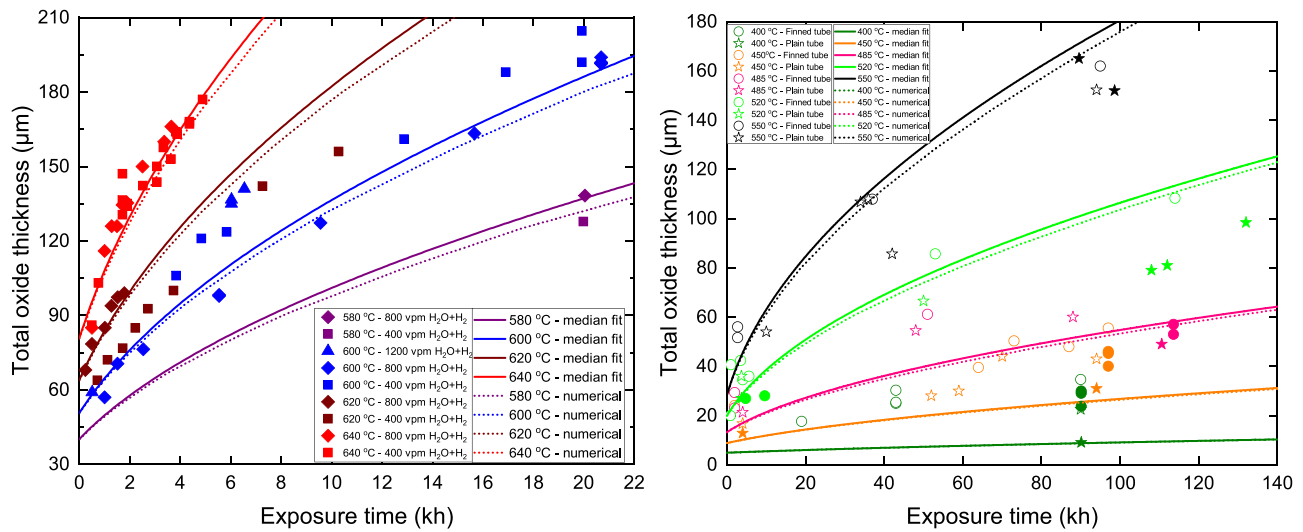
Fig. 4. Comparisons of measured total oxide thickness (solid symbols by this work and hollow symbols from [26]) against analytical fittings (parabolic) and numerical simulations (dashed lines); finned tube samples (solid circles) and plain tube samples (solid star) are exposed at temperatures of 400 °C (olive), 450 °C (orange), 485 °C (pink), 520 °C (green), 550 °C (black), 580 °C (purple), 600 °C (blue), 620 °C (wine) and 640 °C (red); samples above 550 °C are exposed to gas 3 (solid squire), gas 4 (solid diamond) and gas 5 (solid triangle) while samples below 580 °C are exposed to gas 1 (finned samples) and gas 2 (plain tube samples). The median of oxide thickness from measurements is considered here. (For interpretation of the references to colour in this figure legend, the reader is referred to the web version of this article.)
