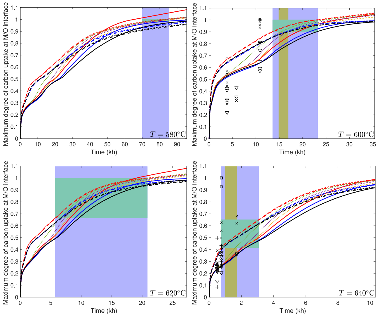
Fig. 10. Predicted maximum degree of carbon uptake of the 9Cr-1Mo alloy taking into account oxidation kinetics with P_C = 1 (red) and P_C = 0 (blue), and without taking into account oxidation kinetics (black); calculations have been done in both 1D (solid lines) and 2D (planar: dashed lines; axisymmetric: short dot lines), with geometry defined in Fig. 12. Values of \alpha_a/V_m and \zeta follow the best fit of for each temperature as outlined in Section 4. The yellow and blue regions cover the range of measured ttb for samples listed in Table 1 and Fig. 3 respectively. The green rectangle shows the range of \eta_C^{\text{eff}} predicted by the 2D axisymmetric model (with P_C = 1 ) in the ttb zone (for the larger dataset). Measured carbon mole fraction at the spinel/substrate interface (converted to the degree of carbon uptake) at 0 ( \square ), 0.5 ( \times ), 1 (+) and 1.5 mm ( \nabla ) away from the fin tip are included, compared to predictions at 0.5 (green dot lines), 1 (purple dot lines) and 1.5 mm (orange dot lines) away from the fin tip. (For interpretation of the references to colour in this figure legend, the reader is referred to the web version of this article.)
