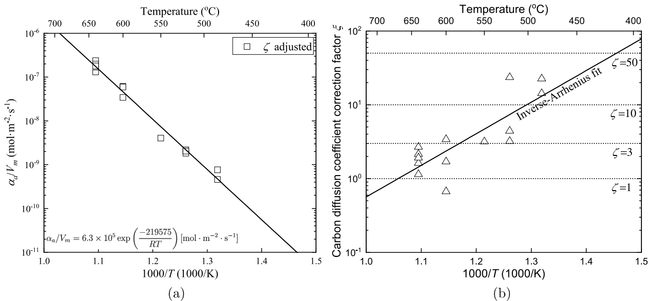
Fig. 9. Derived \alpha_a/V_m (a) and \zeta (b) for each sample by allowing \zeta to be adjusted for each fitting of profiles; black lines show the (inverse) Arrhenius fit of \alpha_a/V_m and \zeta over the temperature. Calculations were done without taking into account oxidation kinetics.
