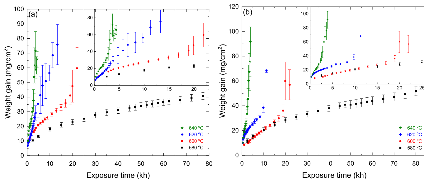
Fig. 3. Weight gains of material HRA1542 exposed to (a) gas composition 3 [8] and (b) gas composition 4 [22], at 580 °C (black), 600 °C (red), 620 °C (blue) and 640 °C (green); one standard deviation from repeated tests is used to evaluate uncertainties. (For interpretation of the references to colour in this figure legend, the reader is referred to the web version of this article.)
