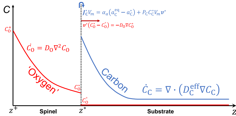
Fig. 8. Illustration of coupling between oxidation with carburisation kinetics. The internal oxidation zone (IOZ, shown in Fig. 6) is omitted here because carbon diffuses through the Cr-depleted matrix of the IOZ rapidly and without reaction; its activity at the IOZ/carburisation zone interface is therefore very little changed from the value at the scale/metal interface.
