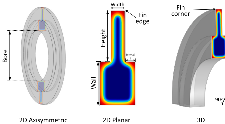
Fig. 12. Geometry of component assumed in the carbon uptake model; oxidation kinetics have been considered for all cases, with the outmost surface (grey) denoting the original gas/substrate interface; the rotational twist representing spiral fins is considered in the 3D case.
