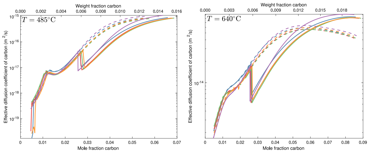
Fig. 7. Calculated effective diffusion coefficient of carbon as a function of total fraction of carbon up to a_C = 1 ; calculations were done either by considering all possible phases (solid lines) or only including the M 23 C 6 type of carbide (dashed lines), with the composition of alloy 277 (blue), 283 (red), 256 (green), HRA1542 (orange) and Fe-9Cr1Mo (purple); the weight fraction of carbon is converted from the molar fraction of carbon based on the Fe-9Cr-1Mo alloy composition. (For interpretation of the references to colour in this figure legend, the reader is referred to the web version of this article.)
