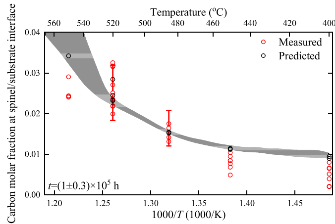
Fig. 11. Comparison of the molar fraction of carbon at the spinel/substrate interface by measurements and predictions; the Arrhenius fit of both \alpha_a/V_m and \zeta are used in the carbon uptake model, with oxidation kinetics considered; the grey region is outlined by predictions considering a 1D geometry corresponding to the fin width or the thickness of the plain tube, for different virgin alloys at around 1 \times 10^5 h; the error of measurement at 485 and 520 °C is estimated based on measurements at the spinel/substrate interface across the plain tube specimen. (For interpretation of the references to colour in this figure legend, the reader is referred to the web version of this article.)
