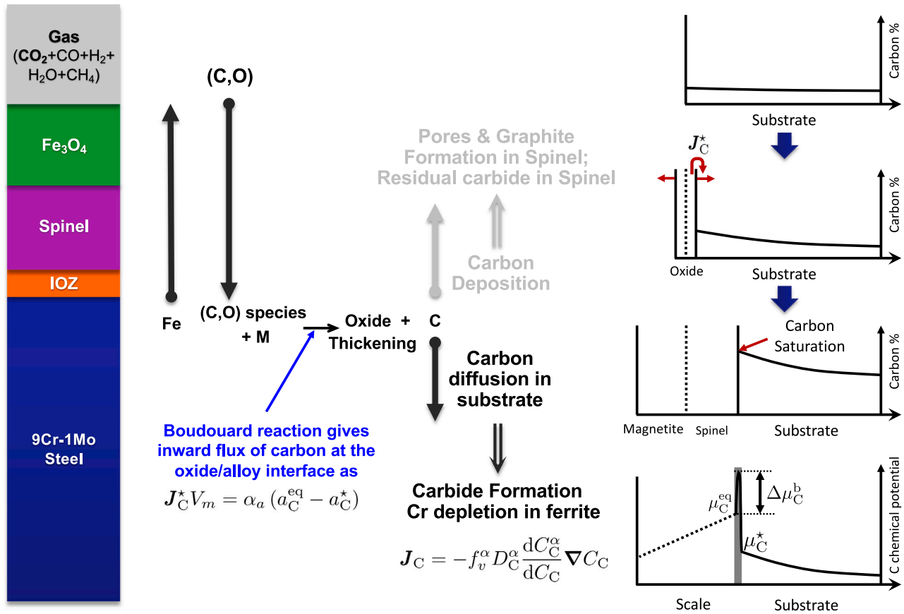
Fig. 6. Illustrations of phase transformations in CO 2 oxidation of 9Cr1Mo steel. The distribution of the chemical potential of carbon is shown at the bottom right.
