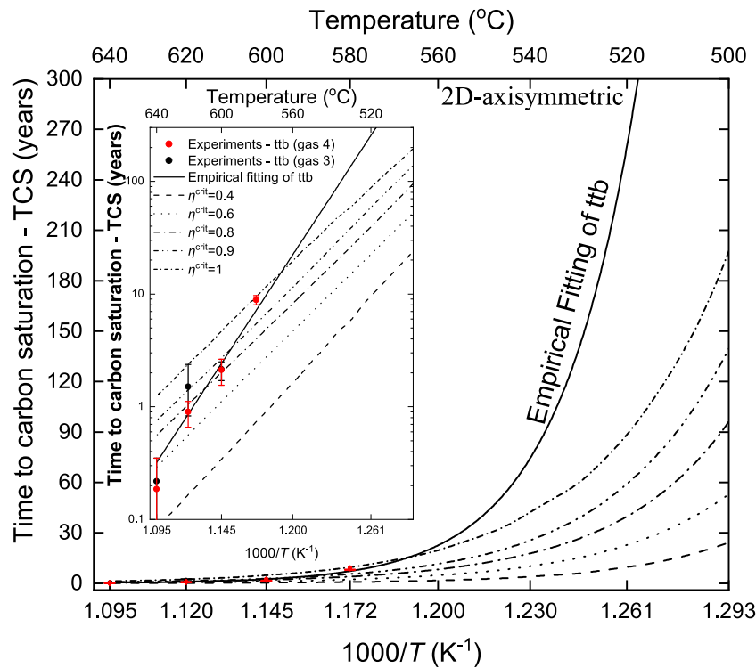
Fig. 14. Predicted time to carbon saturation with different \eta^{\text{crit}} assumed; calculations were done by using the Arrhenius fit of \alpha_a/V_m and inverse-Arrhenius fit of \zeta taking into account oxidation kinetics; a 2D axisymmetric geometry is used. Average ttb (taken as half between TTb and TafterB) measured for samples exposed to gas 3 and gas 4 are represented by black and red circles respectively; The error bar indicates the range of measurements between the minimum TTb and the maximum TafterB. (For interpretation of the references to colour in this figure legend, the reader is referred to the web version of this article.)
