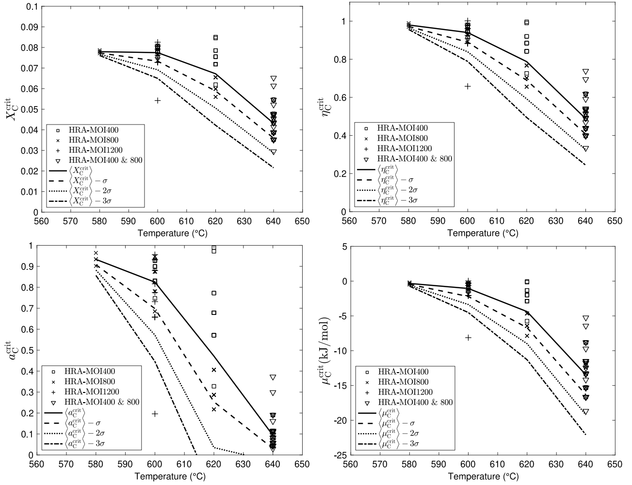
Fig. 13. Calibrated critical X_C , \eta_C , a_C and \mu_C at the spinel/substrate interface; calculations were done taking into account oxidation kinetics.
