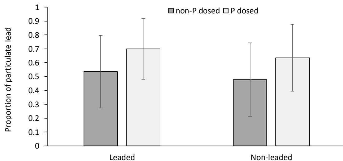
Figure 4. Proportion of particulate lead in all samples for led and unleaded samples, with and without P dosing.
