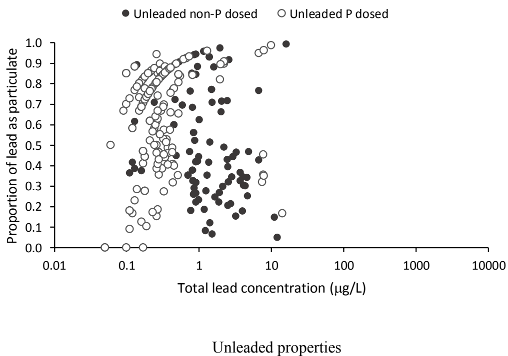
Figure 5. Proportion of particulate lead in samples for unleaded homes, with and without P dosing as a function of the total lead concentration in the sample.
