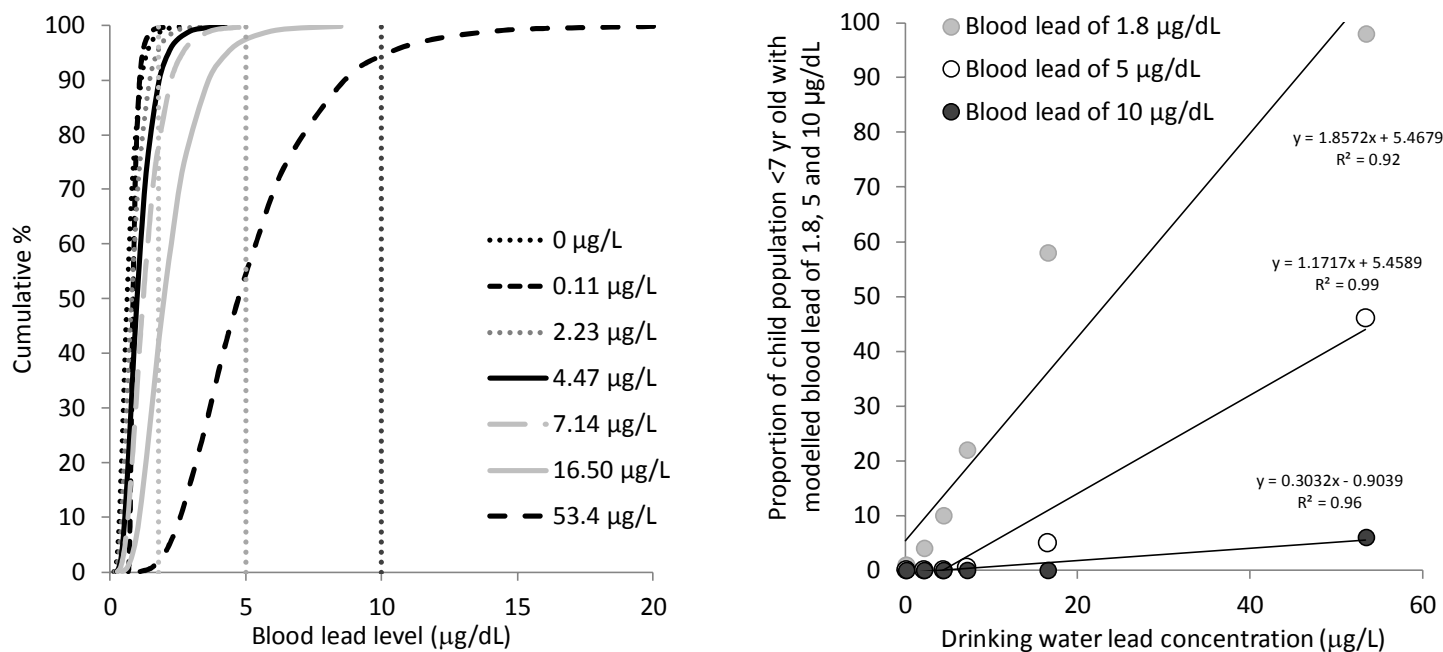
Figure 7. a) Cumulative percentage distribution of estimated BLLs in children <7 years old using the IEUBK model. b) Proportion of population with predicted BLL above 1.8, 5 and 10 µg/dL with increasing tap water concentration. Six tap water lead concentrations have been selected based on data collected during the consumption study.
