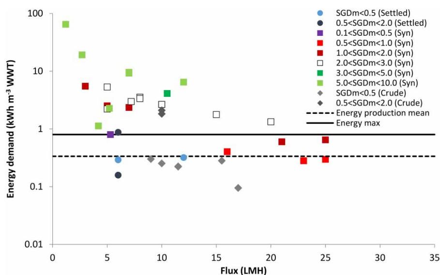
Figure 2 | Comparison of membrane energy demand to the average (0.34 kWh m -3 , dashed line) and maximum (0.80 kWh m -3 , continuous line) energy production reported in the literature to date for anaerobic MBR treating settled wastewater.
