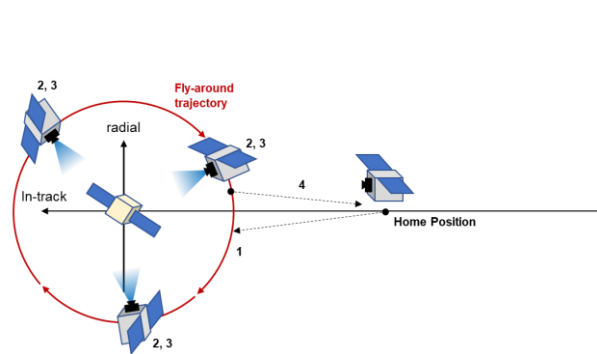
Fig. 4 Fly-around observation close-in CONOPS
