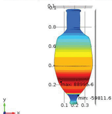
Contour: First principal stress (N/m 2 ) Max/Min Volume: First principal stress (N/m 2 )
