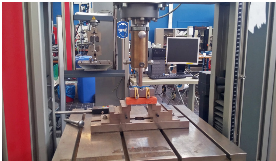
Figure 29: Four-point bending test of test bar with known composition utilizing a custom made pressure block (© TU Delft - Mechanical Test Facility).
