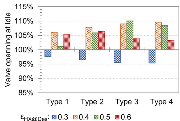
Fig. 21 Valve opening at SLS idle over varying heat exchanger designs and engine types
