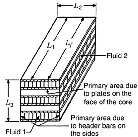
Fig. 5 Plate-fin heat exchanger—crossflow [18]
