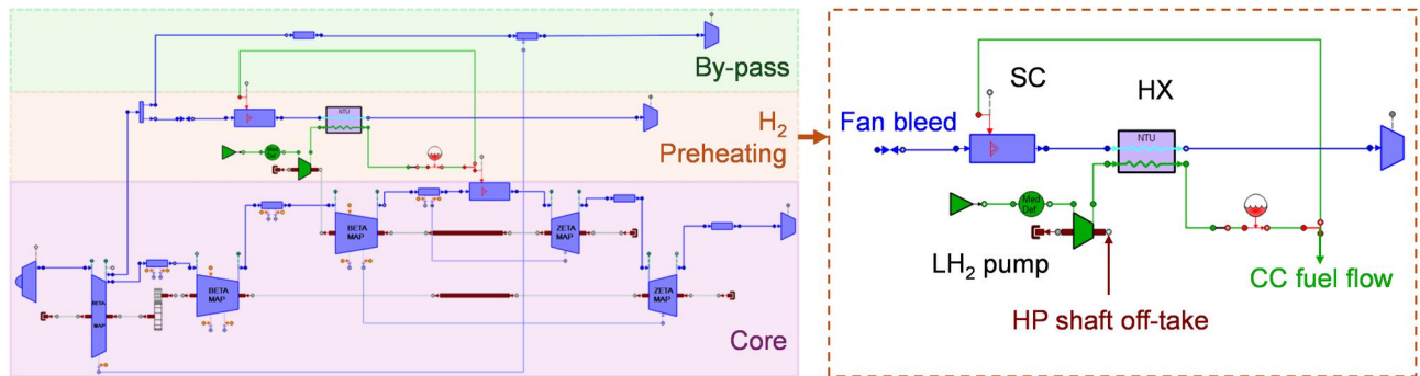
Fig. 14 PHC integrated engine model in PROOSIS
