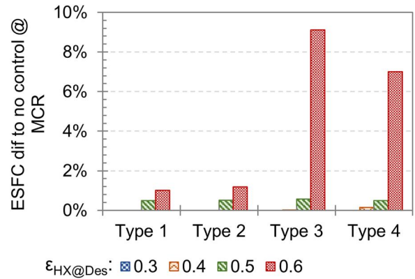
Fig. 19 ESFC difference with and without T_{HX,Hot,out} control
