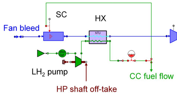
Fig. 1 PHC conditioning system
