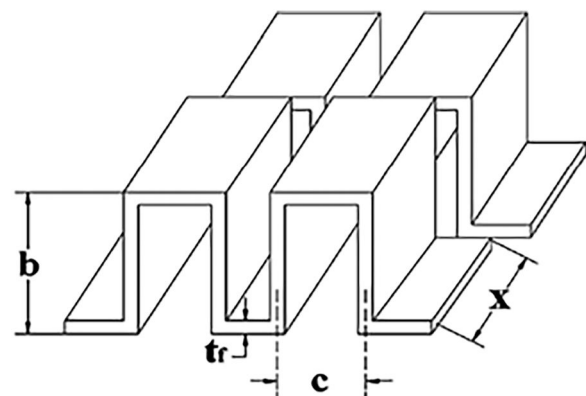
Fig. 6 Offset strip fin geometry [16]
