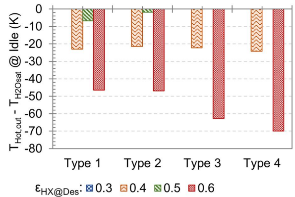
Fig. 20 Condensation temperature margin at SLS idle over varying heat exchanger designs and engine types
