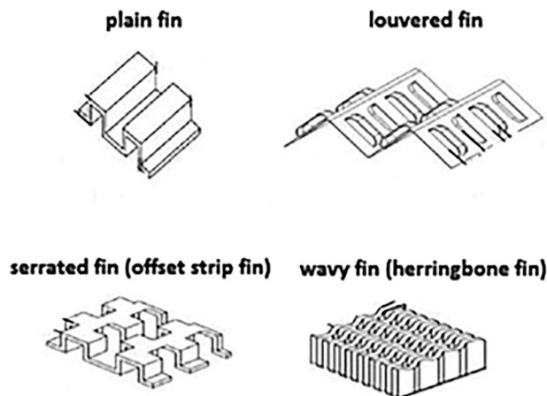
Fig. 4 Common fin configurations [16]
