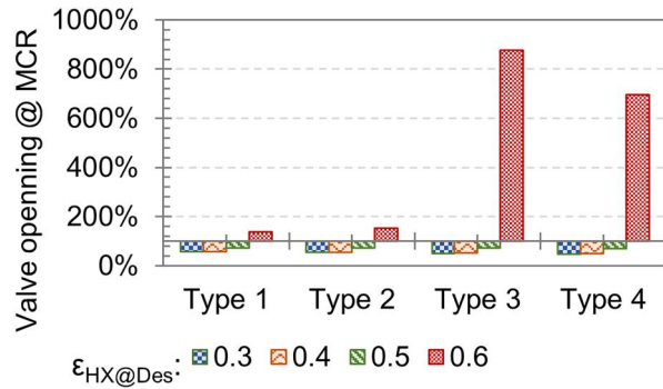
Fig. 16 Valve opening at MCR over varying heat exchanger designs and engine types
