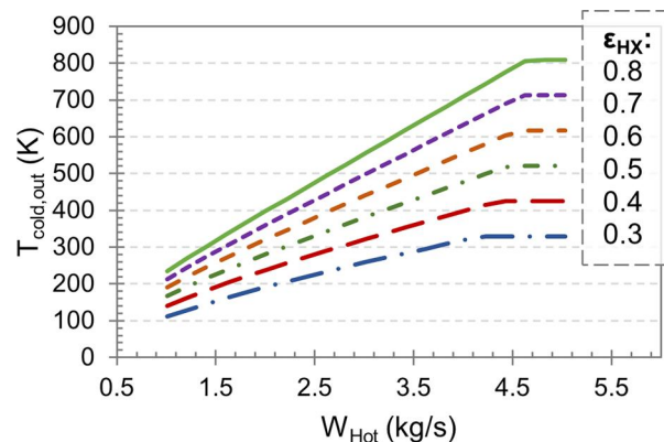
Fig. 10 T_{Cold,out} as a function of W_{Hot} and \epsilon_{HX}
