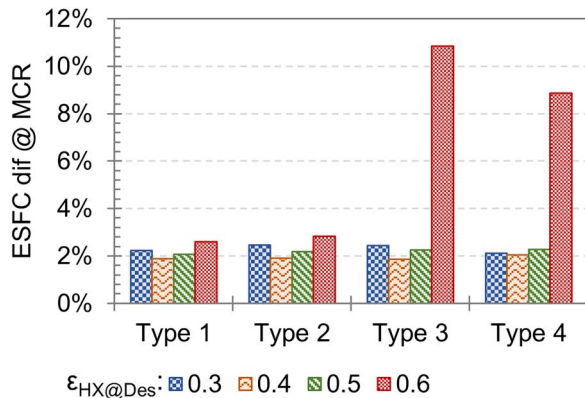
Fig. 18 ESFC difference compared to the respective baseline engine performance over varying heat exchanger designs and engine types
