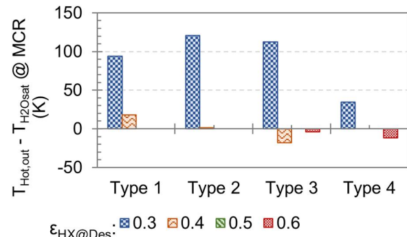
Fig. 15 Condensation temperature margin at MCR over varying heat exchanger designs and engine types
