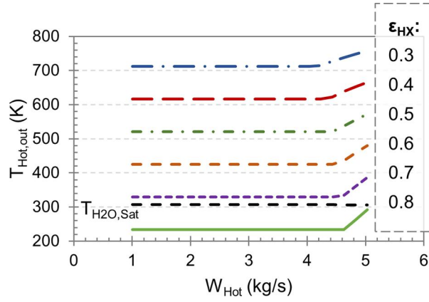
Fig. 11 T_{\text{Hot,out}} as a function of W_{\text{Hot}} and \epsilon_{\text{HX}}
