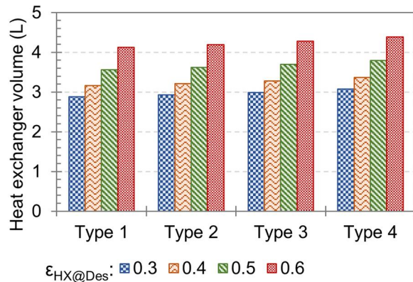
Fig. 22 Heat exchanger volume across the design space
