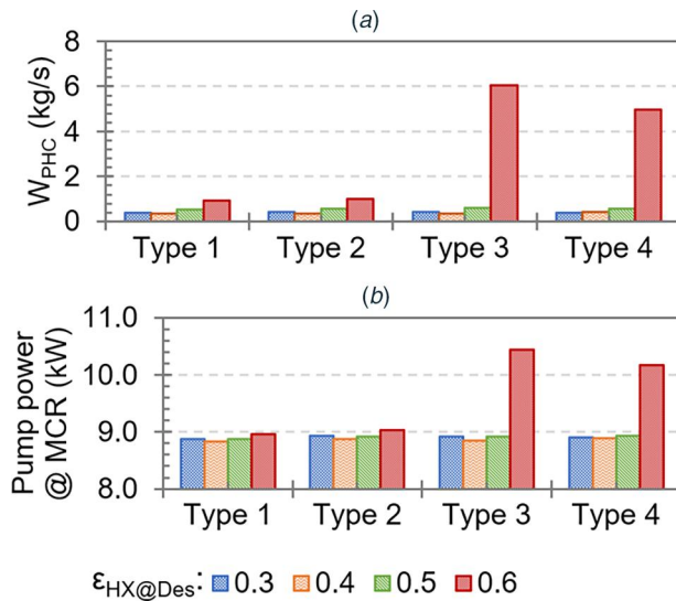
Fig. 17 PHC mass flow (a) and pump power (b) requirements at MCR over varying heat exchanger designs and engine types
