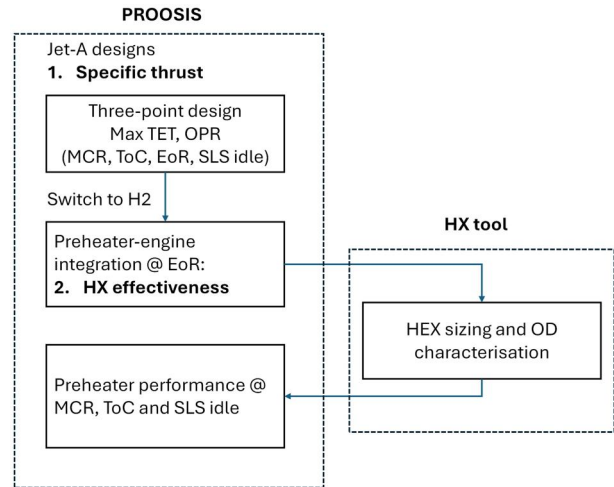
Fig. 2 Workflow overview
