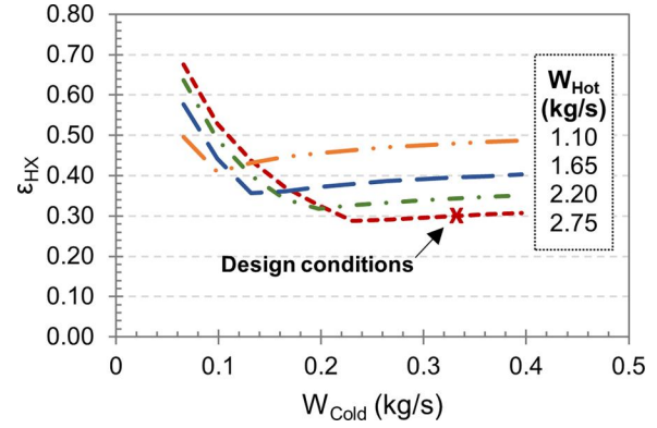
Fig. 13 \epsilon_{\text{HX}} as a function of W_{\text{Cold}} and W_{\text{Hot}}
