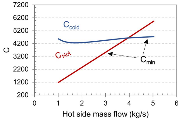
Fig. 12 C_{\text{Cold}} and C_{\text{Hot}} over W_{\text{PHC}} for 0.3 \epsilon_{\text{HX}}
