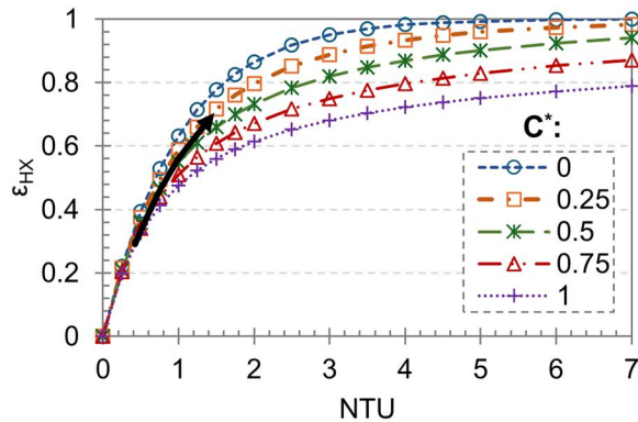
Fig. 8 \varepsilon_{HX} over NTU and C^* for cross flow heat exchangers [17]
