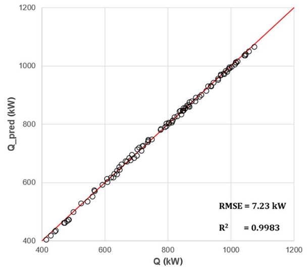
Fig. 9 Heat exchanger regression model result—heat transfer
