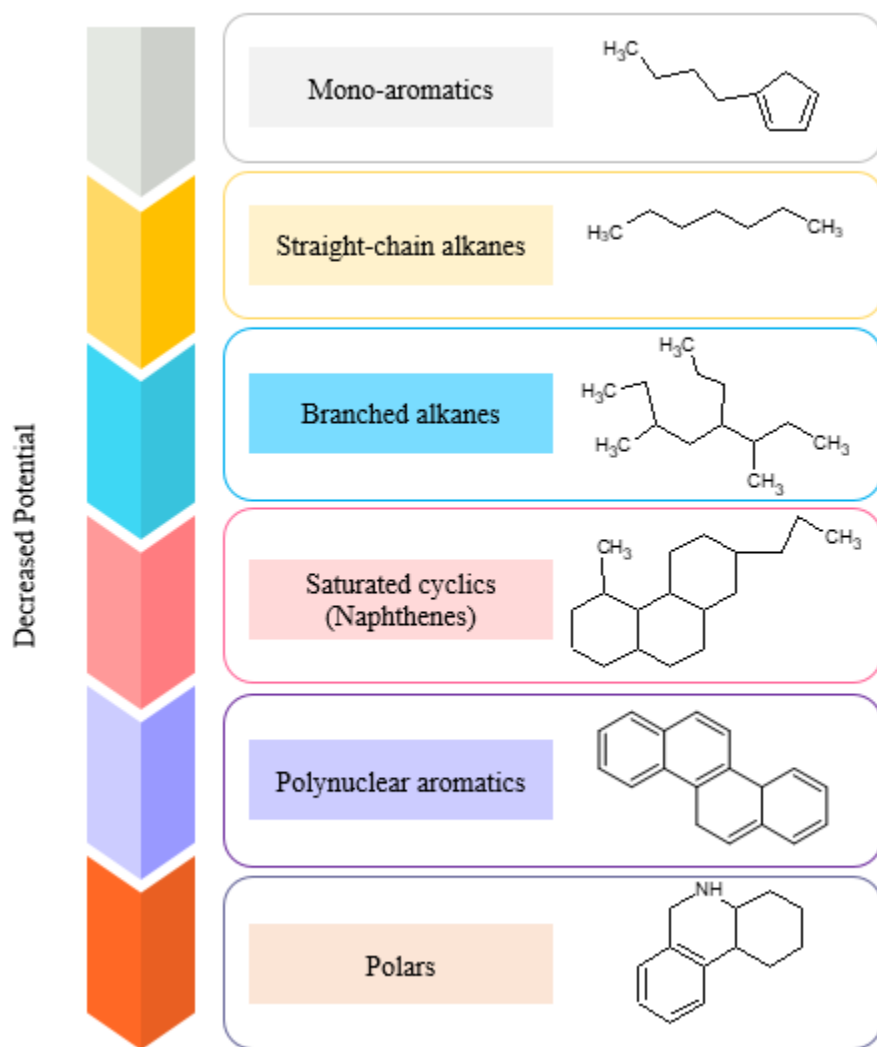
Fig. 4 Biotreatability rate of PHCs (Huesemann, 1994)
