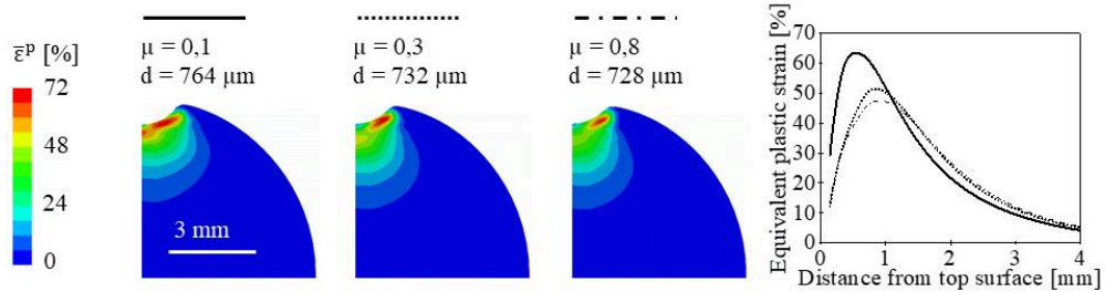
Figure 4: Effect of the friction coefficient ( \mu ) on the equivalent plastic strain of a WAAM Ti-6Al-4V wall after rolling using an inverted-profiled roller with profile radius of 1.5 mm at a rolling load of 75 kN.
