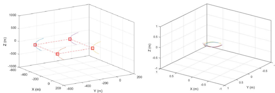
Fig. 14 Spacecraft trajectories with respect to the LVLH coordinate frame (left) and relative position error among spacecraft (right) for the formation reconfiguration maneuver (out-of-plane experiment)
