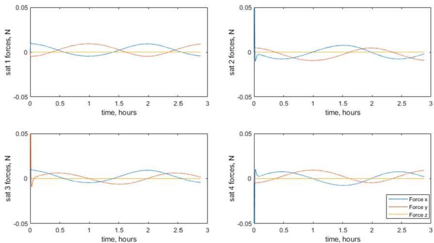
Fig. 9 Forces during the formation-keeping maneuver
