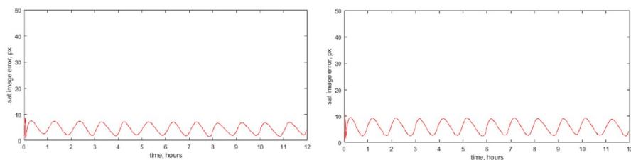
Fig. 20 Image error during the tracking for the hexagonal formation (left) and the triangular formation (right)
