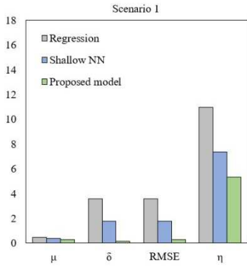
Fig. 10. Comparison of different prediction approaches for the first scenario.
