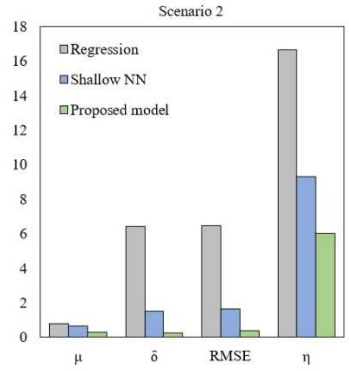
Fig. 11. Comparison of different prediction approaches for the second scenario.
