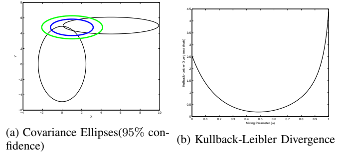
Fig. 4: The fusion of two sensors with dissimilar capabilities and with one measurement biased. Shown are the input covariances (black), the covariance from naive Bayes Fusion (blue) and covariance from MIL fusion (green). On the right hand side is Information Loss as a function of \omega .
