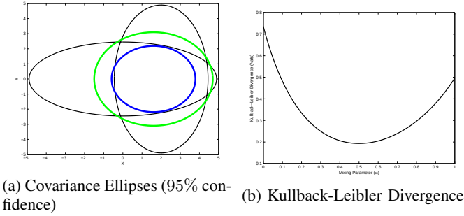
Fig. 2: The fusion of two sensors with similar capabilities, but with one sensor measurement offset. Shown are the input covariances (black), the covariance from naive Bayes Fusion (blue) and covariance from MIL fusion (green). On the right hand side is Information Loss as a function of \omega .
