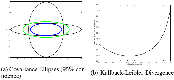
Fig. 3: The fusion of two sensors with dissimilar capabilities. Shown are the input covariances (black), the covariance from naive Bayes Fusion (blue) and covariance from MIL fusion (green). On the right hand side is Information Loss as a function of \omega .
