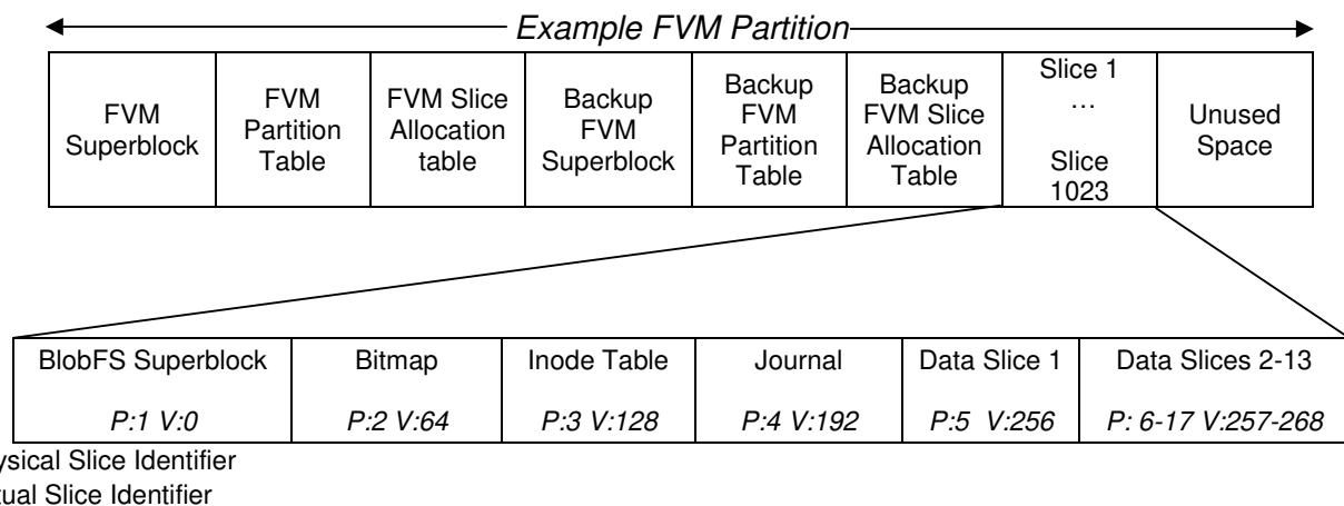
Figure 15: Makeup of BlobFS partition in relation to FVM
