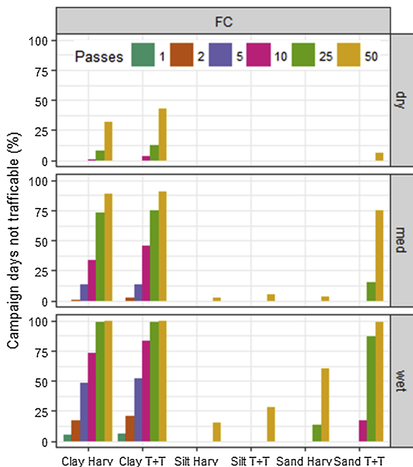
Fig. 6. Proportion of days when the SWC value is not able to support 1, 2, 5, 10, 25 and 50 passes of a harvester (Harv) and a tractor + trailer combination (T + T). This is shown for rainfall scenarios for a dry, median and wet campaign, for the three field sites and starting the simulation at field capacity (FC).
