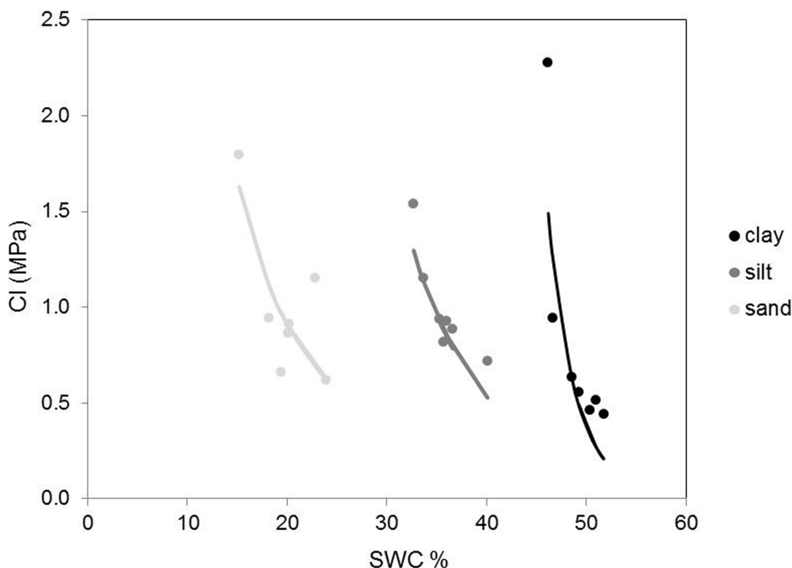
Fig. 3. Calibrations of Cone index ( CI ) using Soil water content ( SWC ) as predictor for three selected field sites. Calibrations represent average CI values between 15 and 30 cm depth and corresponding volumetric SWC derived from tensiometer measurements.
