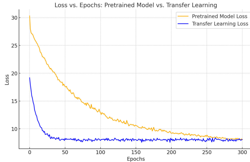
Figure 11. Comparison between the pre-training loss curve and the transfer learning loss curve.
