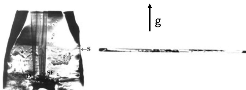
Figure 13. Left: (204) topograph of TNT displaying dislocations (D), stacking faults (SF), (S) indicates where the section topograph was taken. Right: (204) section topograph taken at position (S). 34 Reprinted from J. Cryst. Growth 2003 , 250. Gallagher, H. G.; Vrcelj, R. M.; Sherwood, J. N. The crystal growth and perfection of 2,4,6-trinitrotoluene, 486–498, Copyright (2003), with permission from Elsevier.
