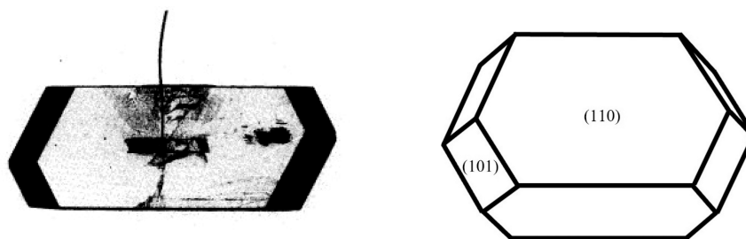
Figure 6. Left: Good quality crystal of PETN; Right: Morphology. 18 Reprinted from J. Cryst. Growth , 1984 , 67, Halfpenny, P. J.; Roberts, K. J.; Sherwood, J. N. Dislocations in energetic materials. I. the crystal growth and perfection of pentaerythritol tetranitrate (PETN), 202–212, Copyright (1984), with permission from Elsevier.
