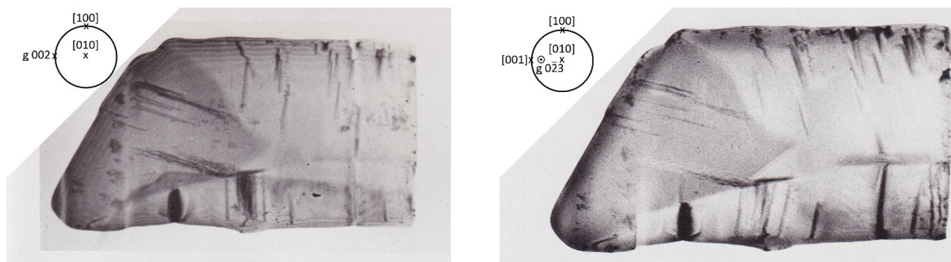
Figure 4. X-ray topographs of an RDX crystal: (a) (002) reflection; (b) (023) reflection.
