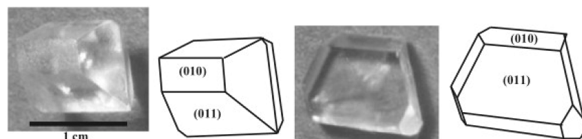
Figure 9. Prismatic and tabular crystals of HMX with associated morphologies. 25 Reprinted from J. Cryst. Growth , 2017, 475, Gallagher, H. G.; Sherwood, J. N.; Vrcelj, R. M. The growth and perfection of \beta -cyclotetramethylene-tetranitramine (HMX) studied by laboratory and synchrotron X-ray topography, 192–201, Copyright (2017), with permission from Elsevier.
