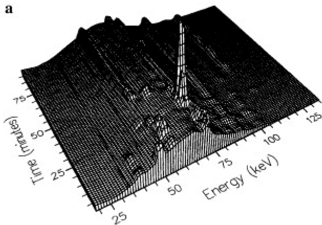
Figure 14. EDXRD traces of TNT precipitating from acetone. Reproduced from ref 33.
