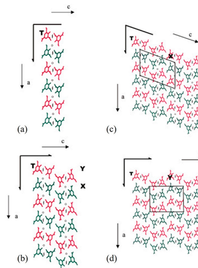
Figure 15. Building a TNT crystal, viewed parallel to the b -axis. (a) Stacks of pairs of TNT molecules originated at T translated along the a -glide plane. (b) Stacks of two pairs of molecules translated along the c -glide plane. (c) Placement of the next “stacks” at X to create the monoclinic form. (d) Alternative placement of the next “stacks” at Y to create the orthorhombic form. Reproduced from ref 35.
