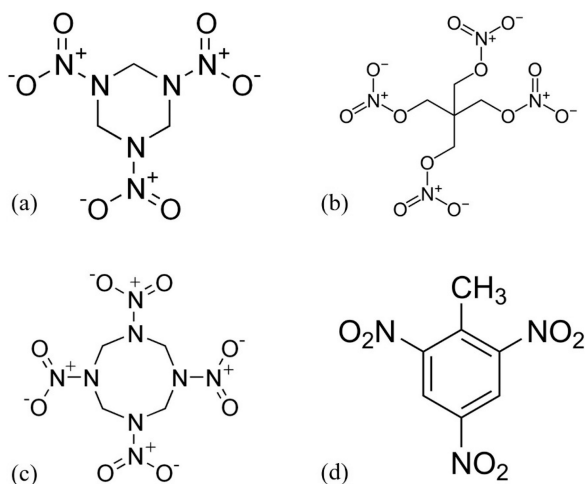
Figure 1. Molecular structures of (a) RDX, (b) PETN, (c) HMX, and (d) TNT.
