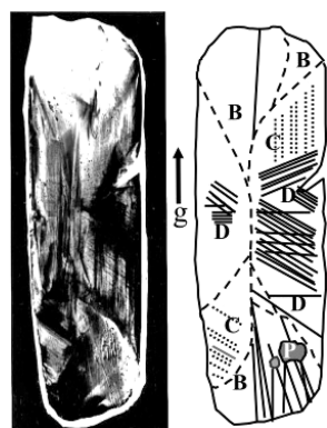
Figure 10. Left: (02\bar{2}) topograph of a (01\bar{1}) slice of a tabular crystal. Right: Schematic showing the complex nature of the growth sectors and their defect content. 25 Reprinted from J. Cryst. Growth , 2017, 475, Gallagher, H. G.; Sherwood, J. N.; Vrcelj, R. M. The growth and perfection of \beta -cyclotetramethylene-tetranitramine (HMX) studied by laboratory and synchrotron X-ray topography, 192–201, Copyright (2017), with permission from Elsevier.
