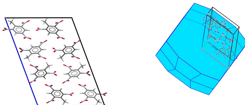
Figure 11. Crystal structure and calculated BFDH morphology of monoclinic TNT.
