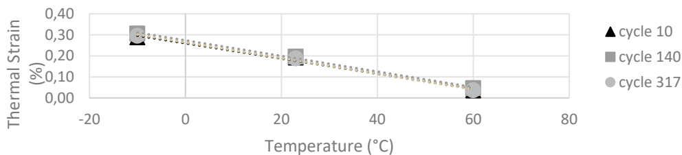
Figure 4: Average thermal strain measurements of 3 shims at thermal cycling intervals during 3 individual cycles
