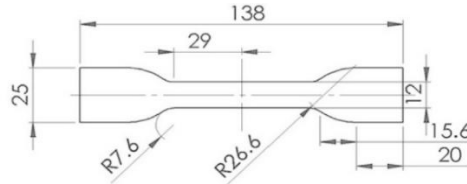
Figure 1: Dimensions (mm) of free film samples
