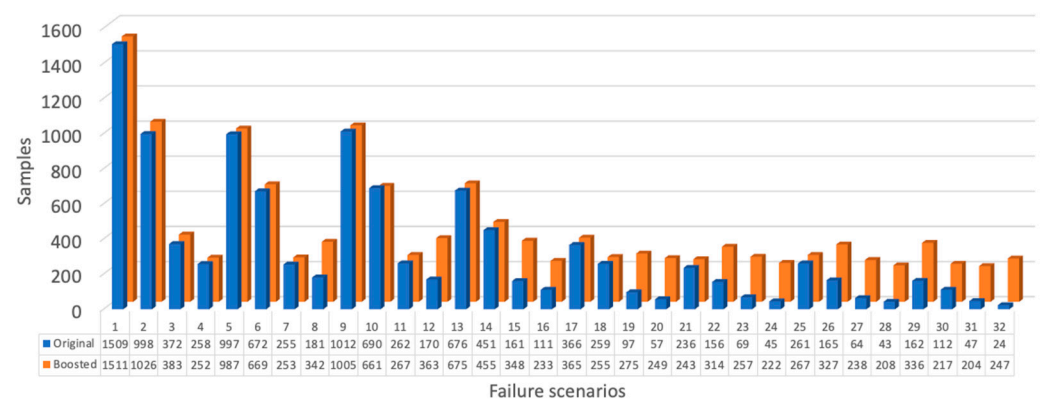
Figure 5. Distribution of the training data.
