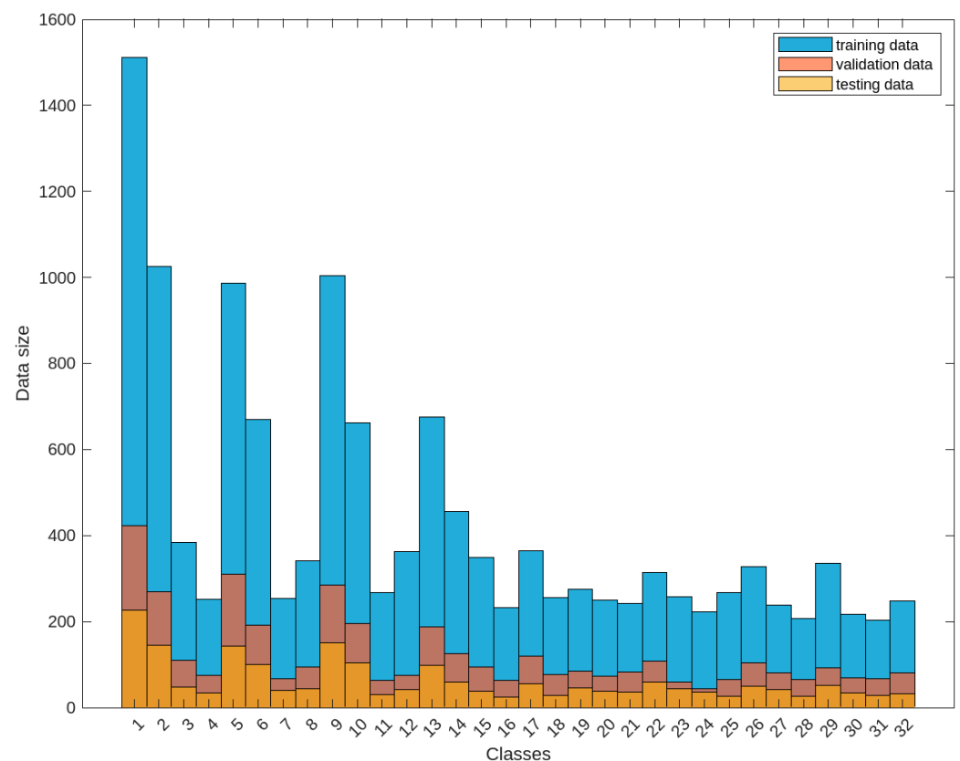
Figure 9. Distribution of training, testing, and validation datasets.
