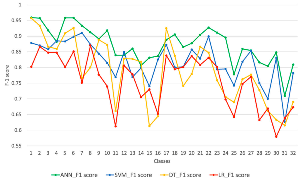
Figure 11. F-1 score of the four algorithms across the 32 classes.
