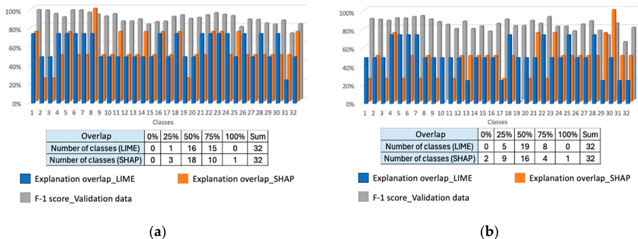
Figure 15. The interpretability of two black-box algorithms: (a) ANN; (b) SVM.
