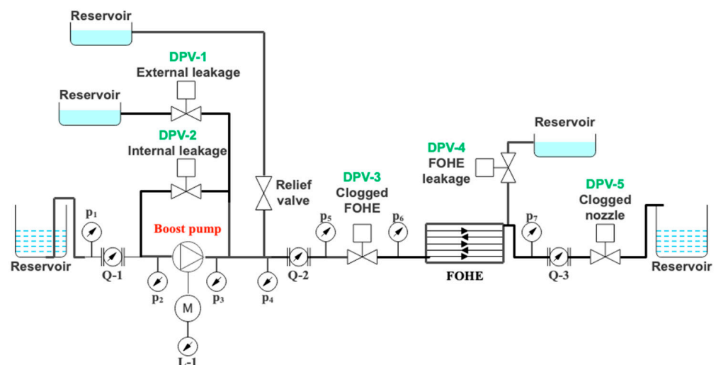
Figure 1. The schematic of the fuel rig.
