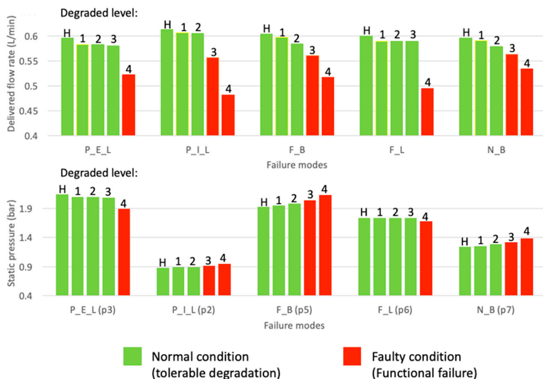
Figure 3. Failure modes' impact on the system's behaviour.
