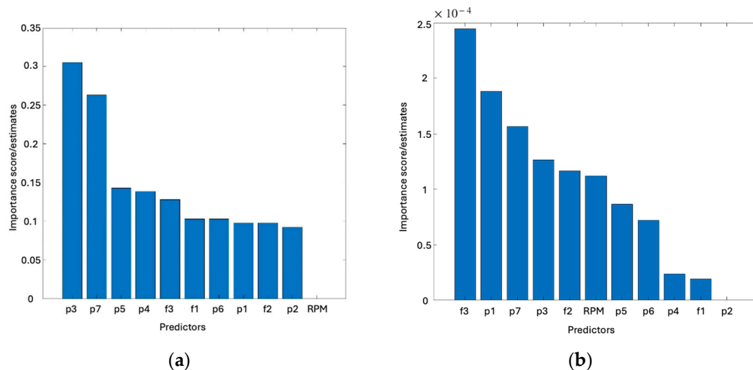
Figure 4. Feature importance rankings: (a) minimum redundancy maximum relevance; (b) tree-based method.
