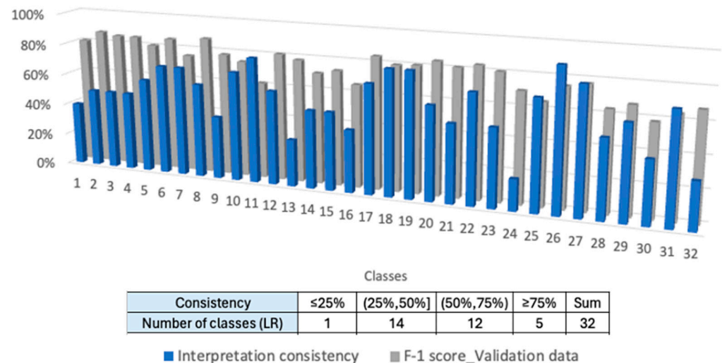
Figure 13. The interpretability of multinomial logistic regression.
