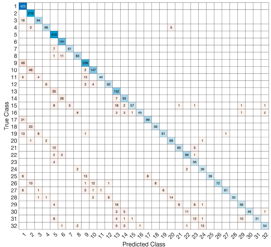
Figure 12. Confusion matrix of the SVM.
