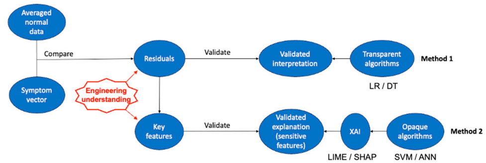
Figure 7. The process of validating explanations with engineering understanding.
