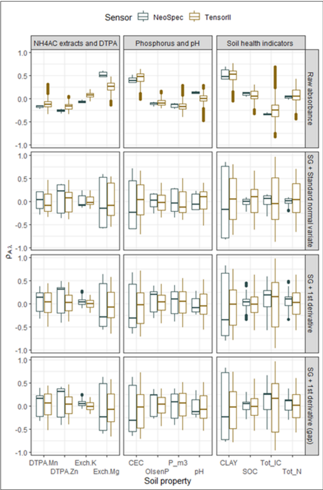
Fig. 4. Correlation boxplot of each soil properties with spectra pre-processing techniques (SG → Savitzsky-Golay smoothing) at each wavelength by the scanning instrumentation (Neospec → Neospectra, Tensor-II → Bruker Tensor 27). The lower and upper limits of each box are the 25th and 75th percentiles, the tails show the correlation range, the dots represent outliers and the horizontal line in each box represents the median.
