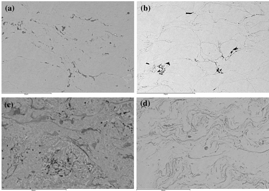
Fig. 4 Representative microstructures of different as-sprayed HVOF coatings. The images have been selected to illustrate the variations in coating microstructures observed. a Ni–50Cr, b FeCrAl, c \text{Cr}_3\text{C}_2 –NiCr matrix, d alloy 625 NiCrMo(Nb+Ta)
