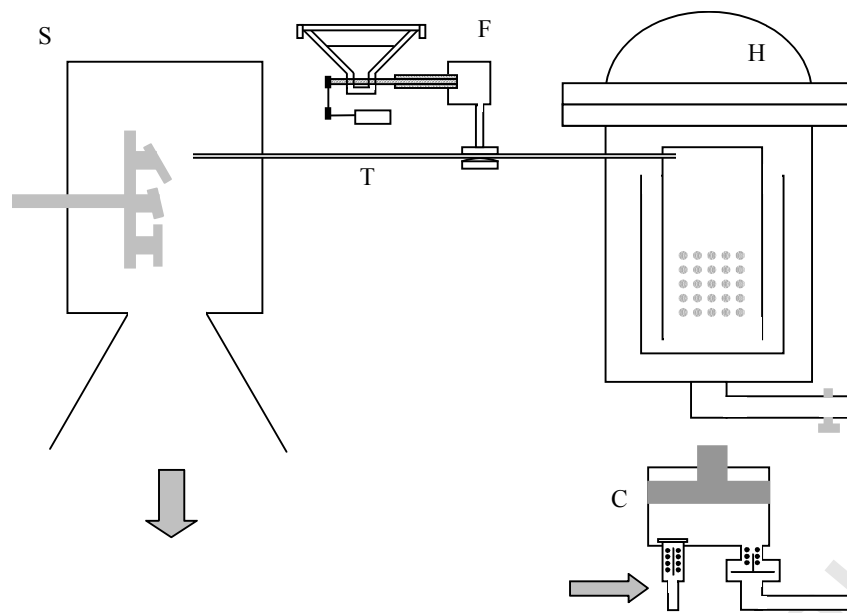
Figure 1: Schematic of the erosion rig.
