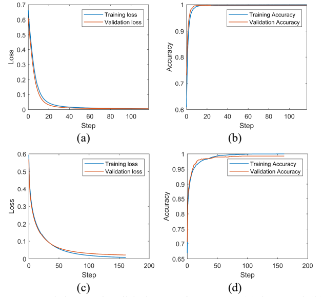
Fig. 9. Training and validation performance: (a) loss and (b) accuracy for the echo window classification model; (c) loss and (d) accuracy for the image quality assessment model
