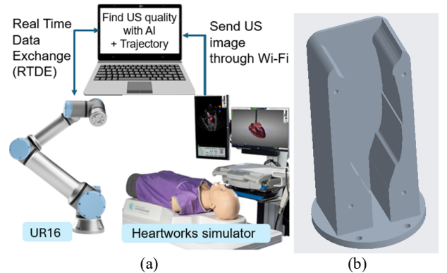
Fig. 3. (a) Echo-Robot hardware setup architecture; (b) the design of the probe end effector
