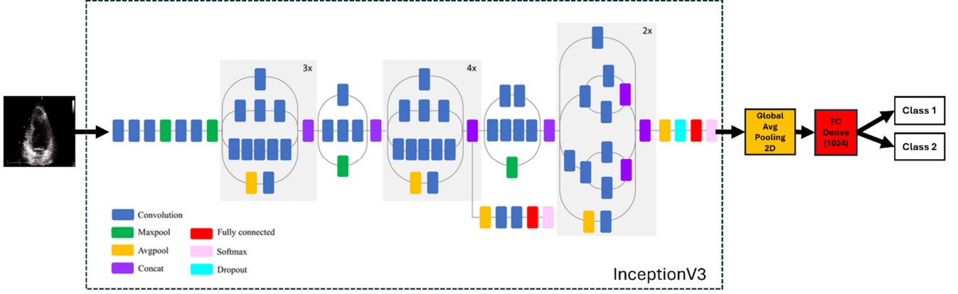
Fig. 5. Diagram of the InceptionV3 models used in this work. Class 1 and Class 2 refer to ‘good’ and ‘bad’ as well as ‘A4Ch’ and ‘A2Ch’ labels.
