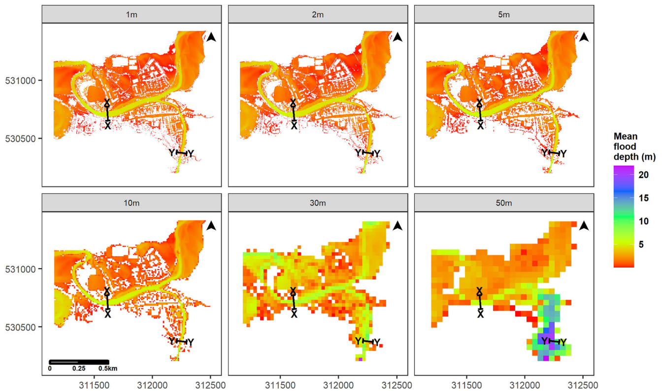
Fig. 8. Flood inundation maps produced using uniform DEMs ranging from 1 m to 50 m.
