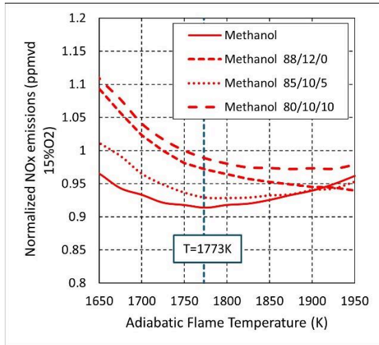
FIGURE 12: IMPACT OF METHANOL COMPOSITION ON \text{NO}_x EMISSIONS FOR A PERFECTLY STIRRED REACTOR FOR 15ms RESIDENCE TIME NORMALISED BY THE VALUE FOR METHANE. (METHANOL COMPOSITION: METHANOL/WATER/ETHANOL IN VOL%).
