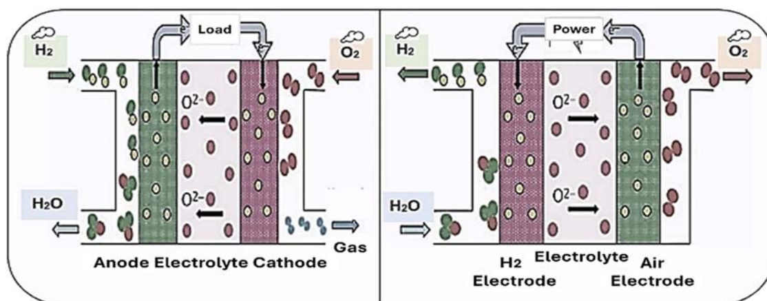
FIGURE 2 SOFC (left) and SOEC (right) operating systems (Pandiyan et al., 2019).
