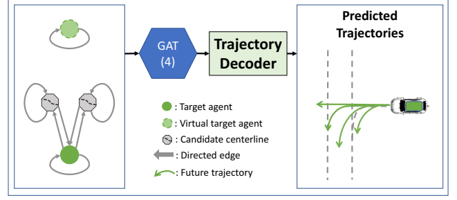
Fig. 4. Map-adaptive trajectory decoder. After encoding, we apply another GAT on the graph with edges shown in the left block of this figure. This is to distribute the target agent's feature to the CCL nodes and let the target agent node reconsider its options (CCLs). Then we apply a trajectory decoder to output the final multimodal prediction.
