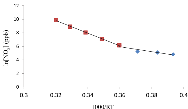
Figure 2. Arrhenius plot of \text{NO}_x evolution from nitrocellulose at different temperatures.
