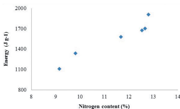
Figure 1. Plot of decomposition energy vs nitrogen content for nitrocellulose samples listed in Table 2.
