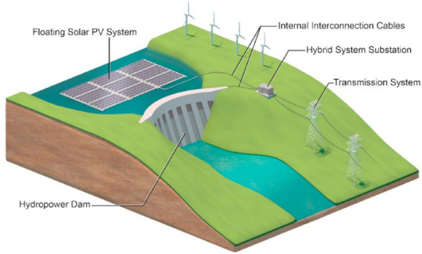
Fig. 1. Schematic of a hybrid FPV-hydropower system [9]
