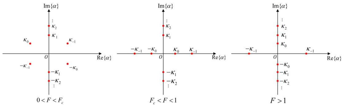
274 Fig. 3. Distribution of the roots of K_1(\alpha, F) = 0 in the entire complex plane of \alpha .
