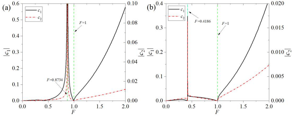
Fig. 10. Coefficients |c_1| and |c_2| versus F ( D = 0.0001 ). (a): Clamped edge; (b) Simply supported edge.
