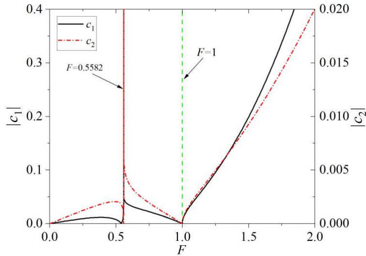
Fig. 8. Coefficients |c_1| and |c_2| versus F . ( D = 0.001 , edge condition: simply supported)
