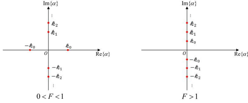
Fig. 4. Distribution of the roots of K_2(\alpha, F) = 0 in the entire complex plane of \alpha .
