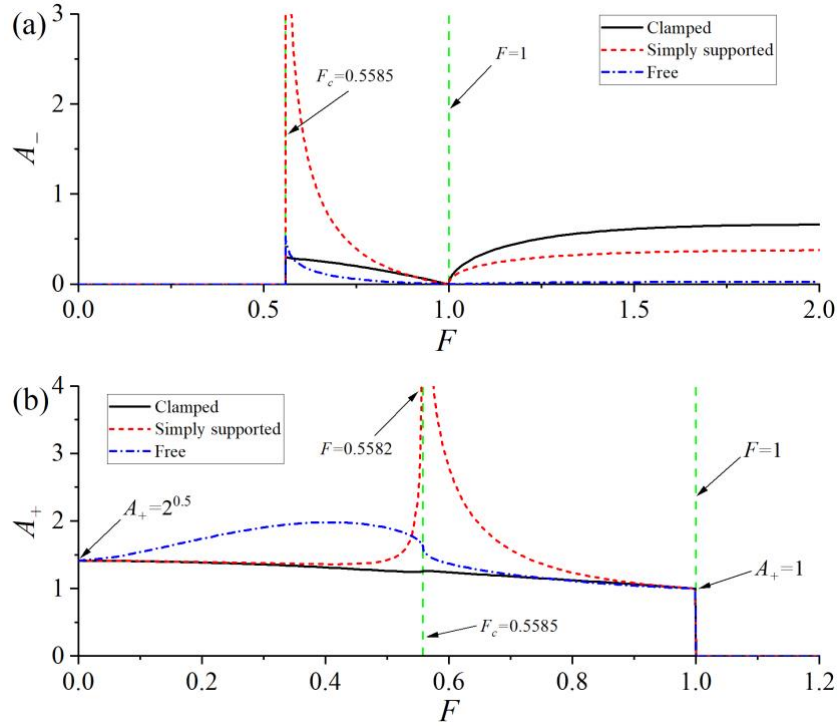
418 419 Fig. 7. The amplitude of the waves at x = \pm\infty versus F ( D = 0.001 )
