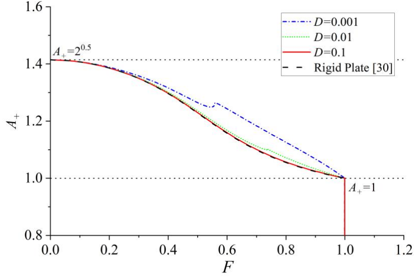
417 Fig. 6. The amplitude of the wave at x = +\infty versus F . (Clamped edge condition)
