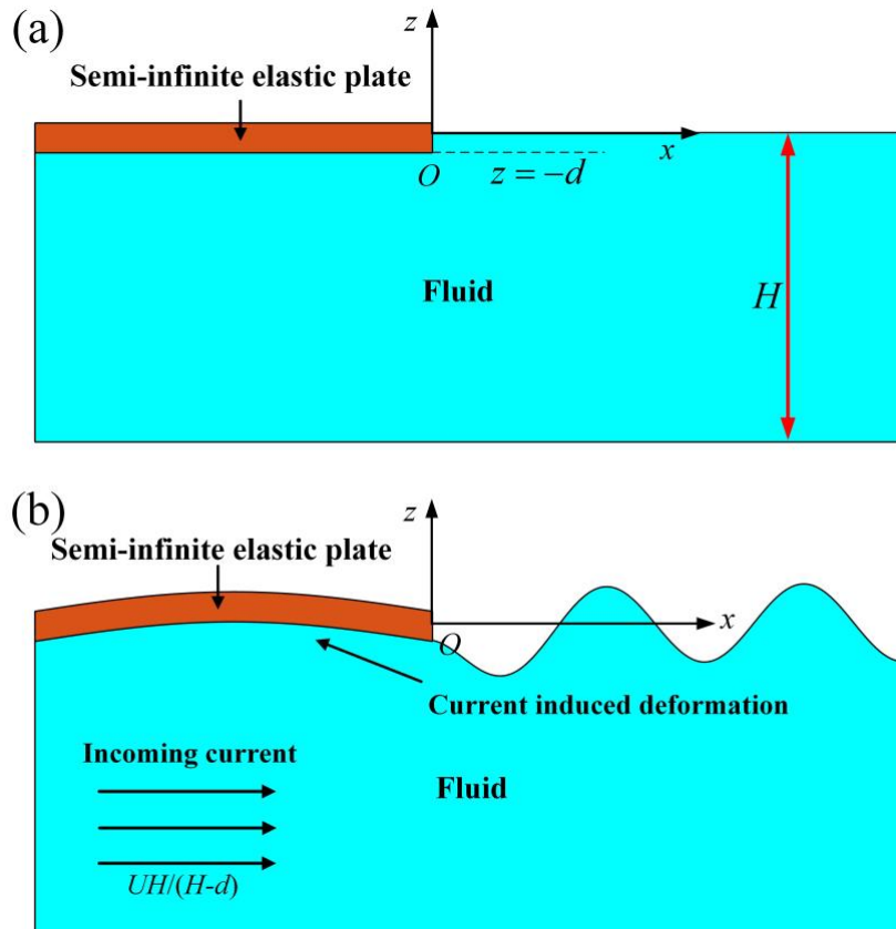
Fig. 2. Schematic of the case: the interaction between a semi-infinite elastic plate with an incoming current. (a). Before the current coming into the system; (b). A steady state after the fluid and structural domains are coupled.
