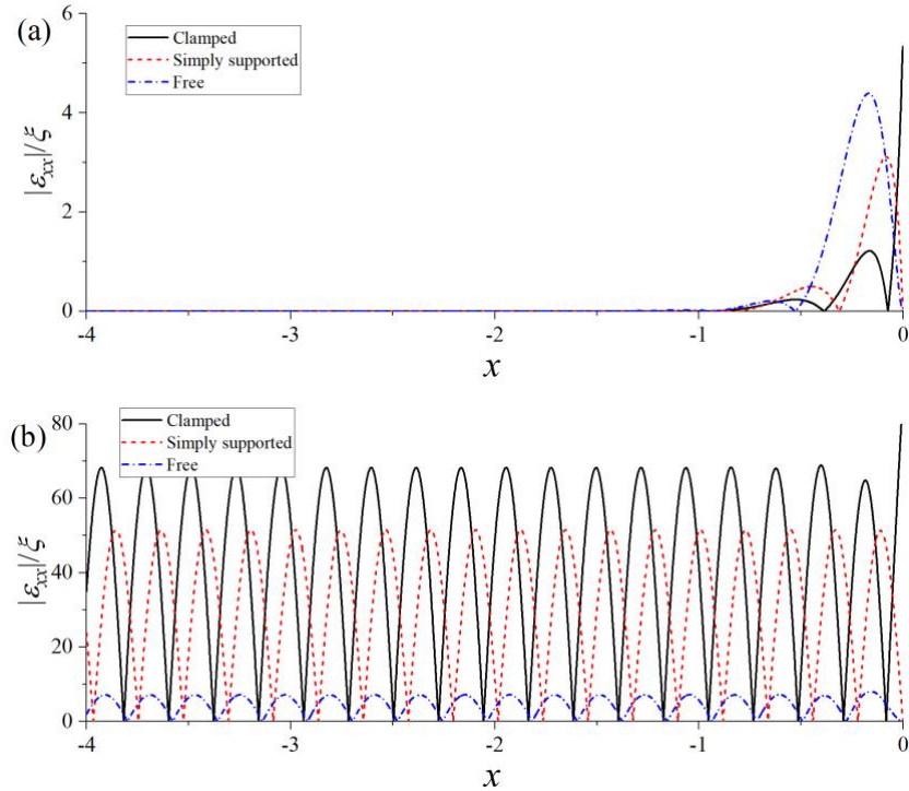
Fig. 15. The principal strain of the elastic plate at two different Froude numbers ( D = 0.0001 , F_c = 0.4189 ). (a): F = 0.2 ; (b) F = 0.6 .
