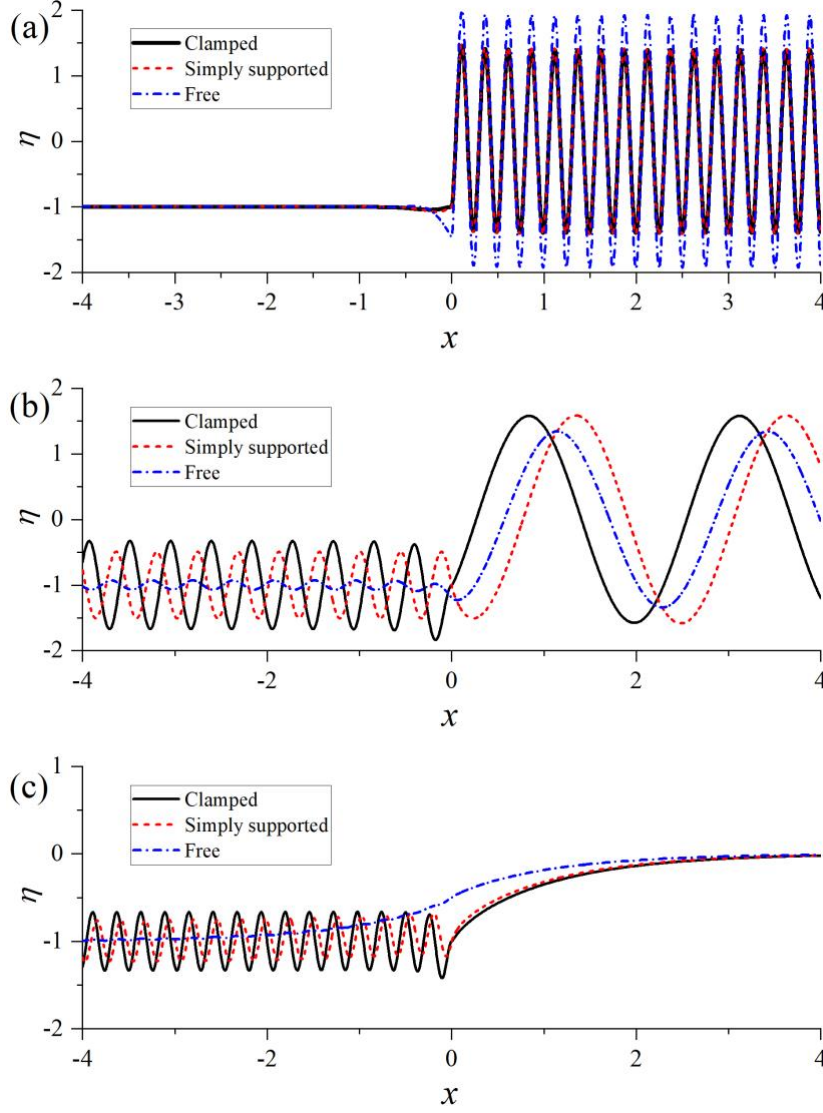
Fig. 13. Wave profiles at three different Froude numbers ( D = 0.0001 , F_c = 0.4189 ). (a): F = 0.2 ; (b) F = 0.6 ; (c) F = 1.2 .
