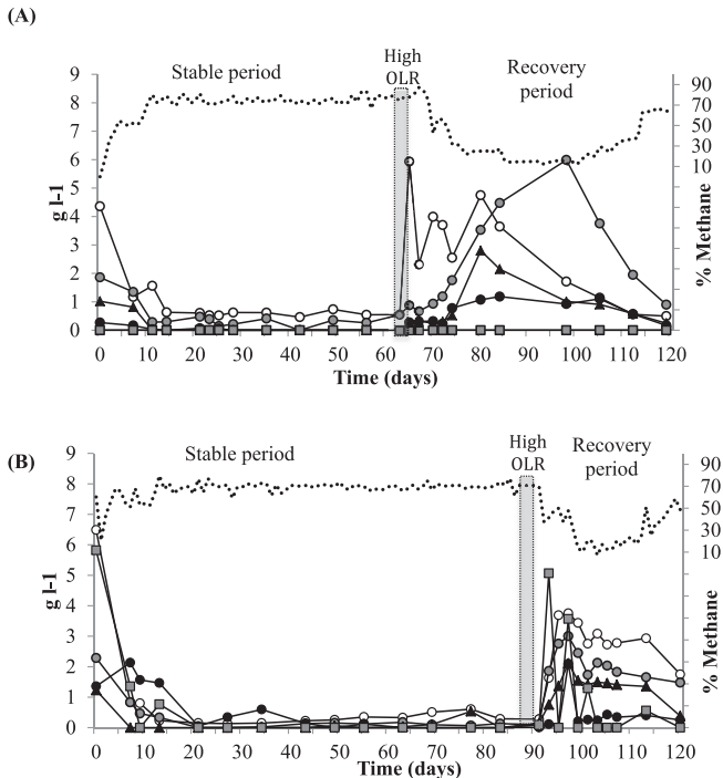
Fig. 1. VFA concentrations and methane content in digesters after one OLR change with glycerol (A) and FOGs (B). Acetic acid (white circles), propionic acid (grey circles), iso-butyric acid (black circles), n-butyric acid (black triangle) and lactic acid (grey squares). Dashed line shows methane content. Triplicate digester average, error bars are not shown to improve legibility.
