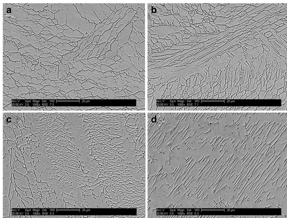
Fig. 9 SEM images. a As-welded. b Post-weld cold rolled. c Post-weld cold rolling followed by laser in first phase. d Post-weld cold rolling followed by laser in second phase
