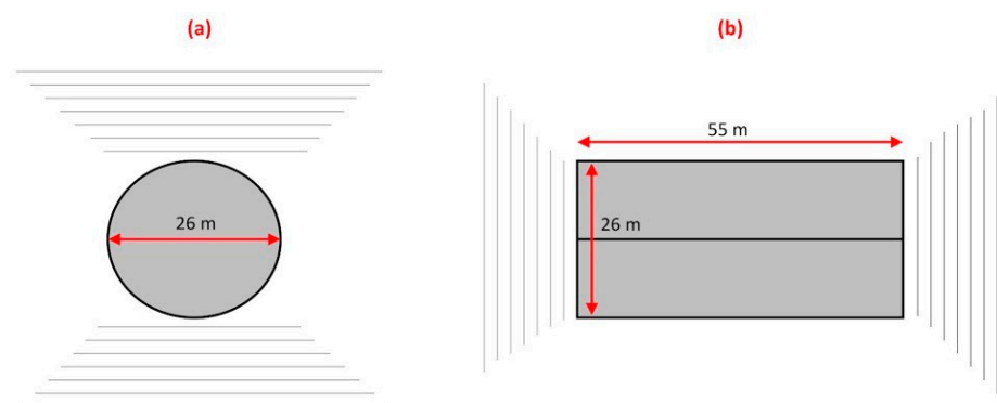
Figure 5. Demonstration of the lines (red) used to determine upwind and downwind measurements for the anaerobic digesters (a) and digestate storage tanks (b). Source: [17].
