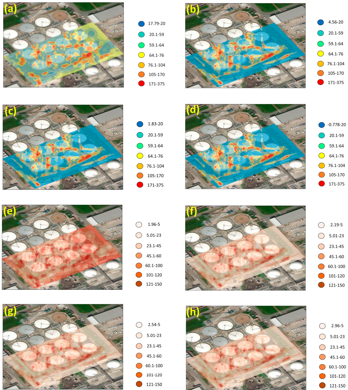
Figure 10. Kriging interpolations and prediction standard error surfaces of vertical path integrated CH 4 concentrations (21 March 2022) for the anaerobic digesters: generated using ArcGIS Pro 2.8. Source: (Esri, 2023). Kriging interpolations: (a) Original data set. U10 CH 4 measurements below the detection level were set to (b) 5 ppm-m, (c) 2.5 ppm-m and (d) 0 ppm-m. Prediction standard error surface: (e) Original data set. U10 CH 4 measurements below the detection level were set to (f) 5 ppm-m, (g) 2.5 ppm-m and (h) 0 ppm-m.
