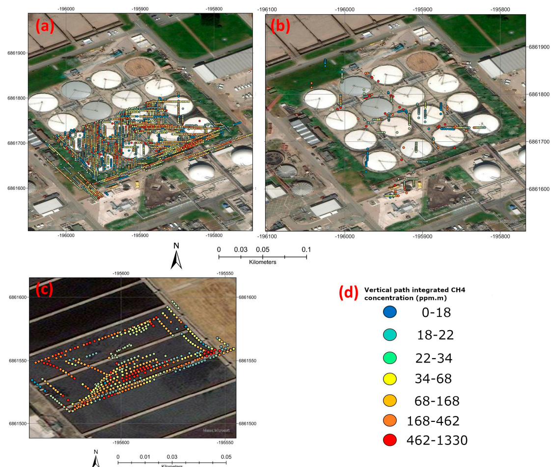
Figure 6. Raw CH 4 measurements registered above the quantification level for the anaerobic digesters (a,b) and the digestate storage tank (c), generated using ArcGIS Pro 2.8 (Esri, USA). Source: [17]. (a) 21 March 2022. (b) 18 May 2022. (c) 4 November 2022. (d) Vertical path integrated CH 4 concentration colour scale in ppm·m. These represent the spatial distribution of vertical column integrated CH 4 concentrations in ppm·m.
