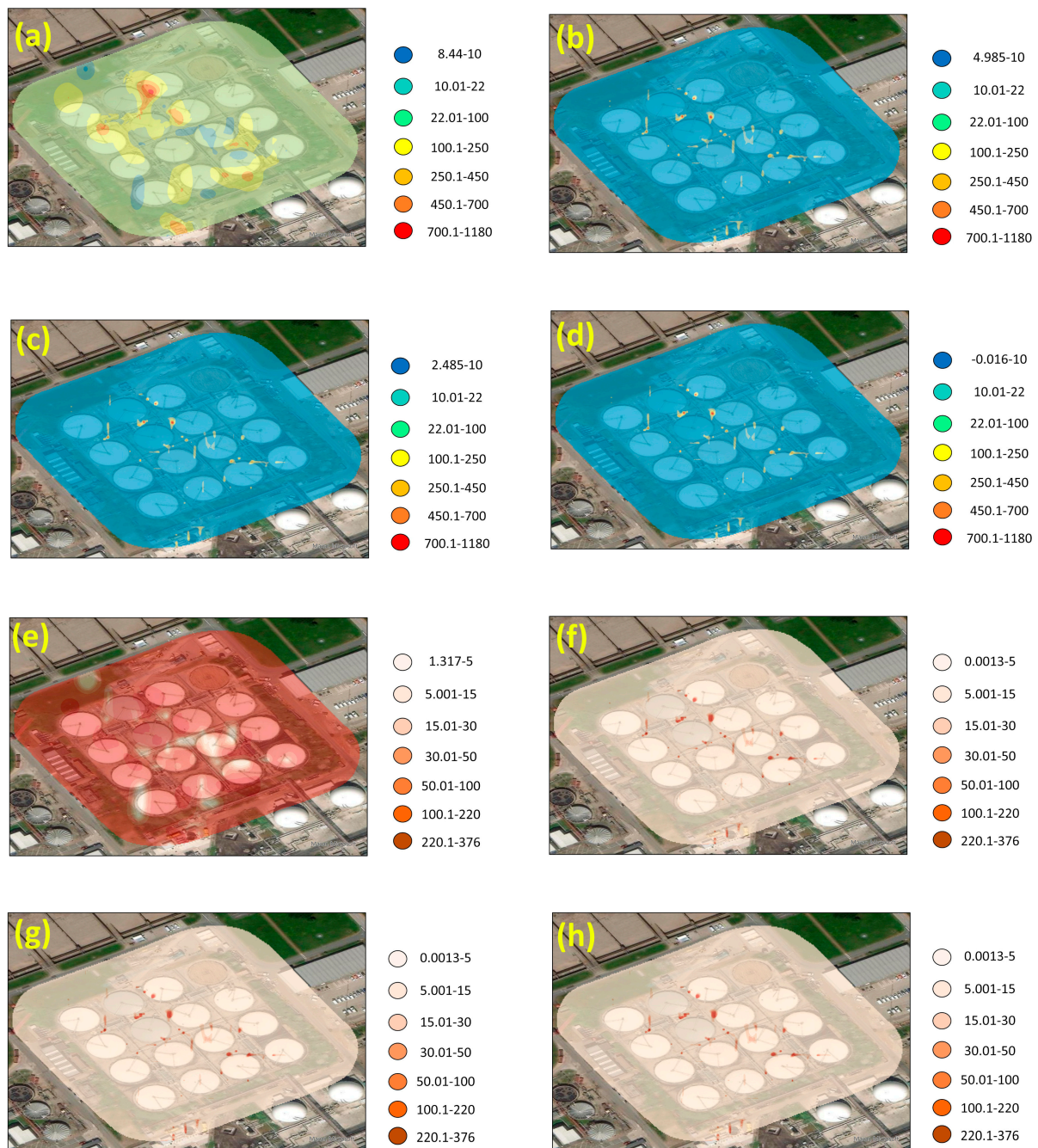
Figure 11. Kriging interpolations and prediction standard error surfaces of vertical path integrated CH 4 concentrations (18 May 2022) for the anaerobic digesters: generated using ArcGIS Pro 2.8. Source: (Esri, 2023). Kriging interpolations: (a) Original data set. U10 CH 4 measurements below the detection level were set to (b) 5 ppm·m, (c) 2.5 ppm·m and (d) 0 ppm·m. Prediction standard error surface: (e) Original data set. U10 CH 4 measurements below the detection level were set to (f) 5 ppm·m, (g) 2.5 ppm·m and (h) 0 ppm·m.
