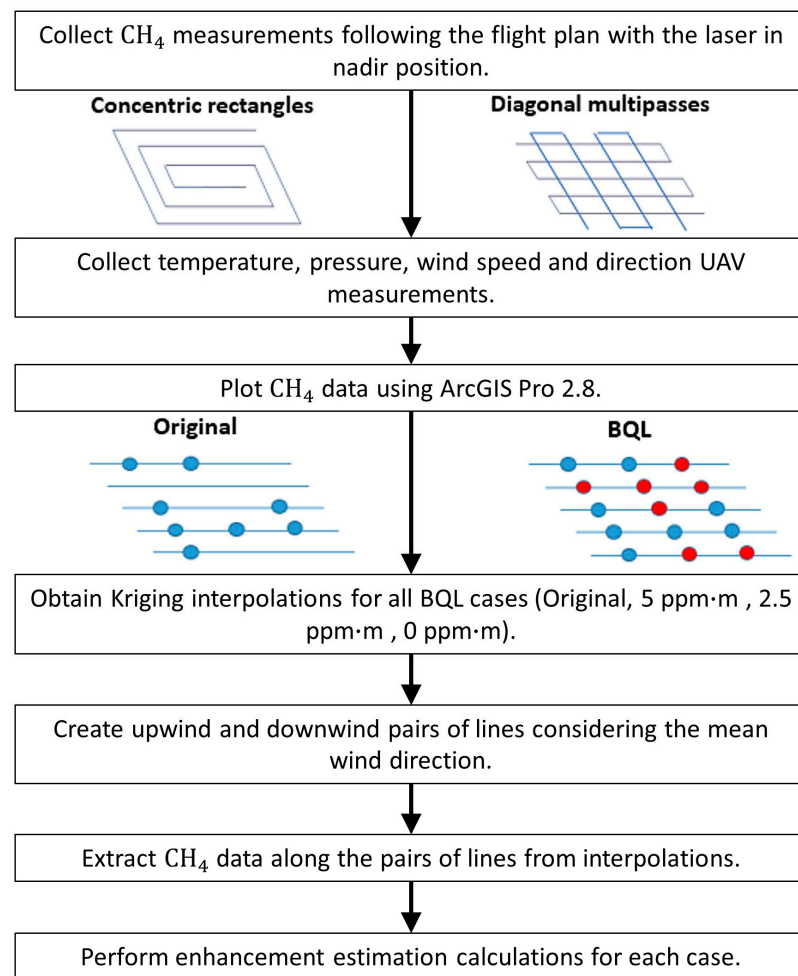
Figure 4. Workflow depicting the data collection and processing followed. BQL stands for below quantification level.
