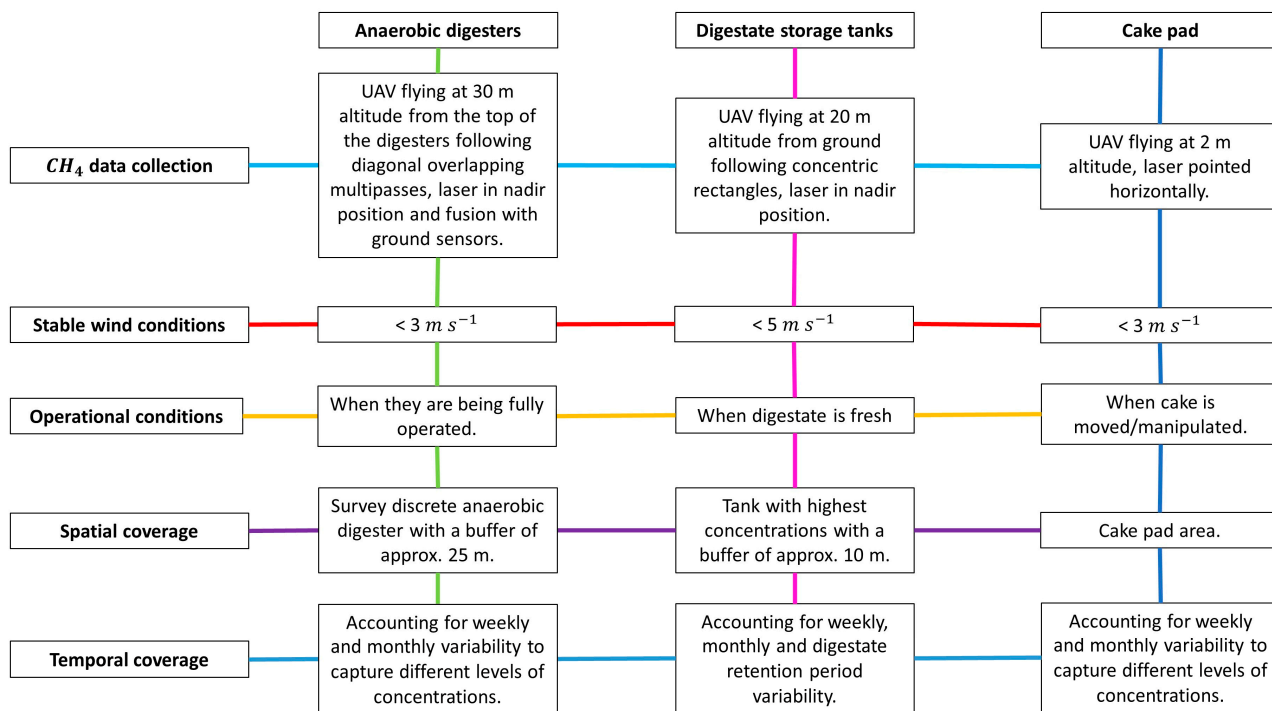
Figure 14. Diagram summarizing recommended data collection strategies based on the U10-UAV sensor thresholds, methodological limitations and results from the ground sensor temporal analysis.
