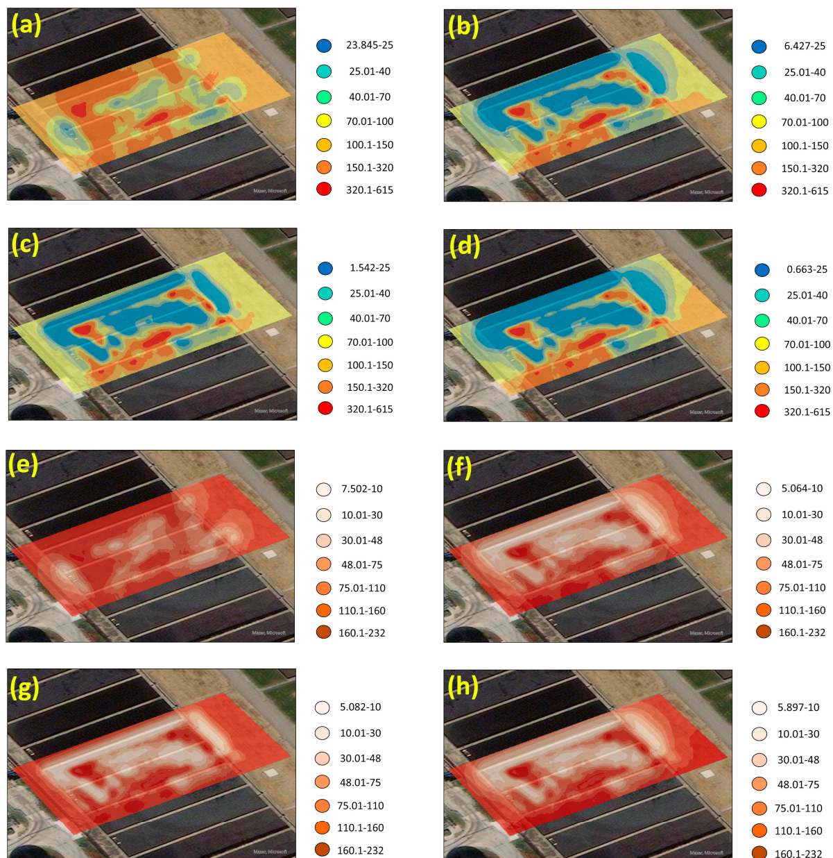
Figure 12. Kriging interpolations and prediction standard error surfaces of vertical path integrated \text{CH}_4 concentrations (4 November 2022) for the digestate storage tanks: generated using ArcGIS Pro 2.8. Source: (Esri, 2023). Kriging interpolations: (a) Original data set. U10 \text{CH}_4 measurements below the detection level were set to (b) 5 ppm·m, (c) 2.5 ppm·m and (d) 0 ppm·m. Prediction standard error surface: (e) Original data set. U10 \text{CH}_4 measurements below the detection level were set to (f) 5 ppm·m, (g) 2.5 ppm·m and (h) 0 ppm·m.
