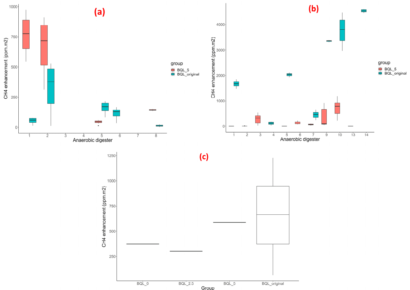
Figure 13. CH 4 enhancement estimations for each anaerobic digester (a,b) and the digestate storage tank (c). The boxes represent the inter quartile range. BQL_5, BQL_2.5 and BQL_0 represent the enhancement obtained when considering all values below quantification level to be 5 ppm·m, 2.5 ppm·m and 0 ppm·m, respectively. For BQL_original, enhancement was calculated with the raw data. (a) 21 March 2022 (b) 18 May 2022 and (c) 4 November 2022.
