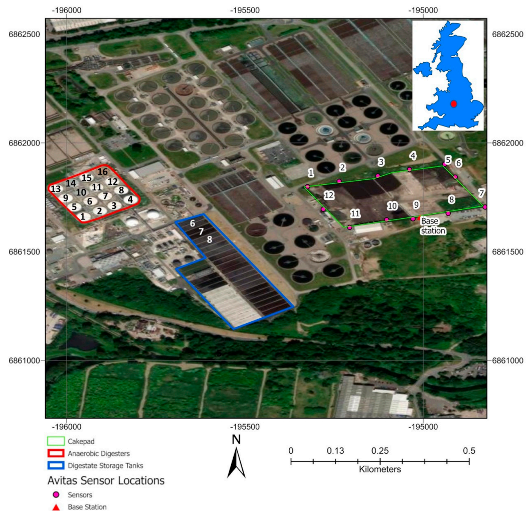
Figure 1. Maps showing the location and distribution of the sludge treatment assets at Minworth WWTP (numbers identify ground sensors along the cake pad area (green polygon) and single units within digestate storage tanks (blue) and anaerobic digesters (red)): generated using ArcGIS Pro 2.8 (Esri, Redlands, CA, USA). Source: [17].
